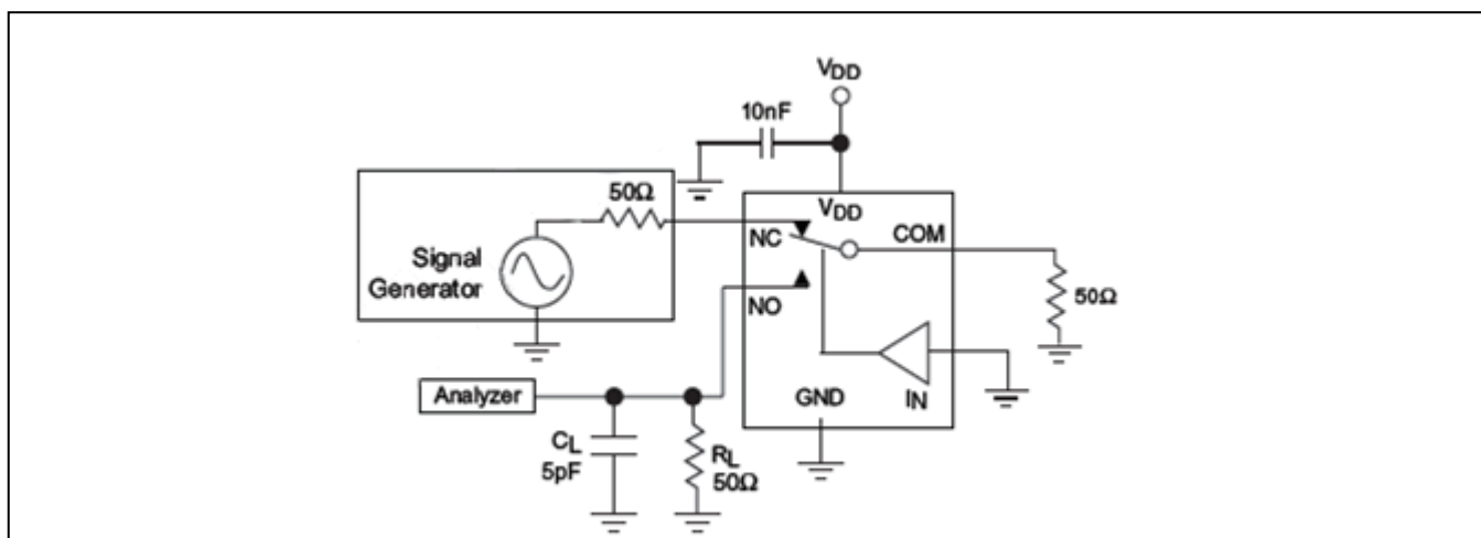
Figure 5. NC-NO Isolation
