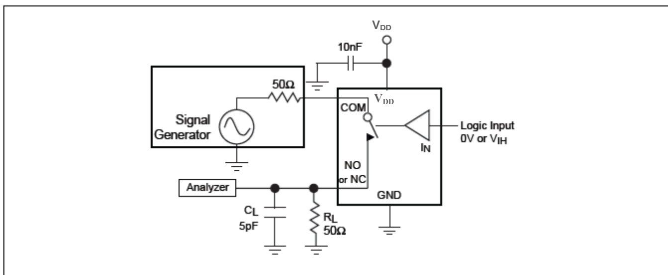
Figure 4. COM-NC/NO Isolation
