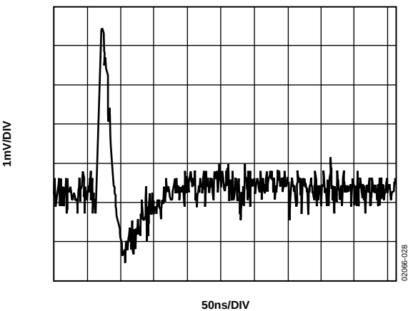
Figure 28. DAC-to-DAC Crosstalk
