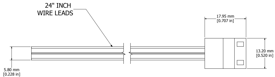
BOTTOM VIEW
