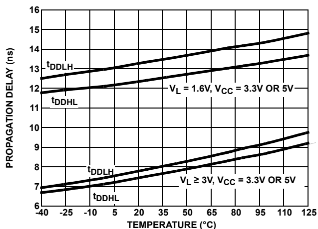
FIGURE 20. DRIVER DIFFERENTIAL PROPAGATION DELAY vs TEMPERATURE (ISL32172E, ISL32174E, ISL32179E, 32Mbps OPTION)
