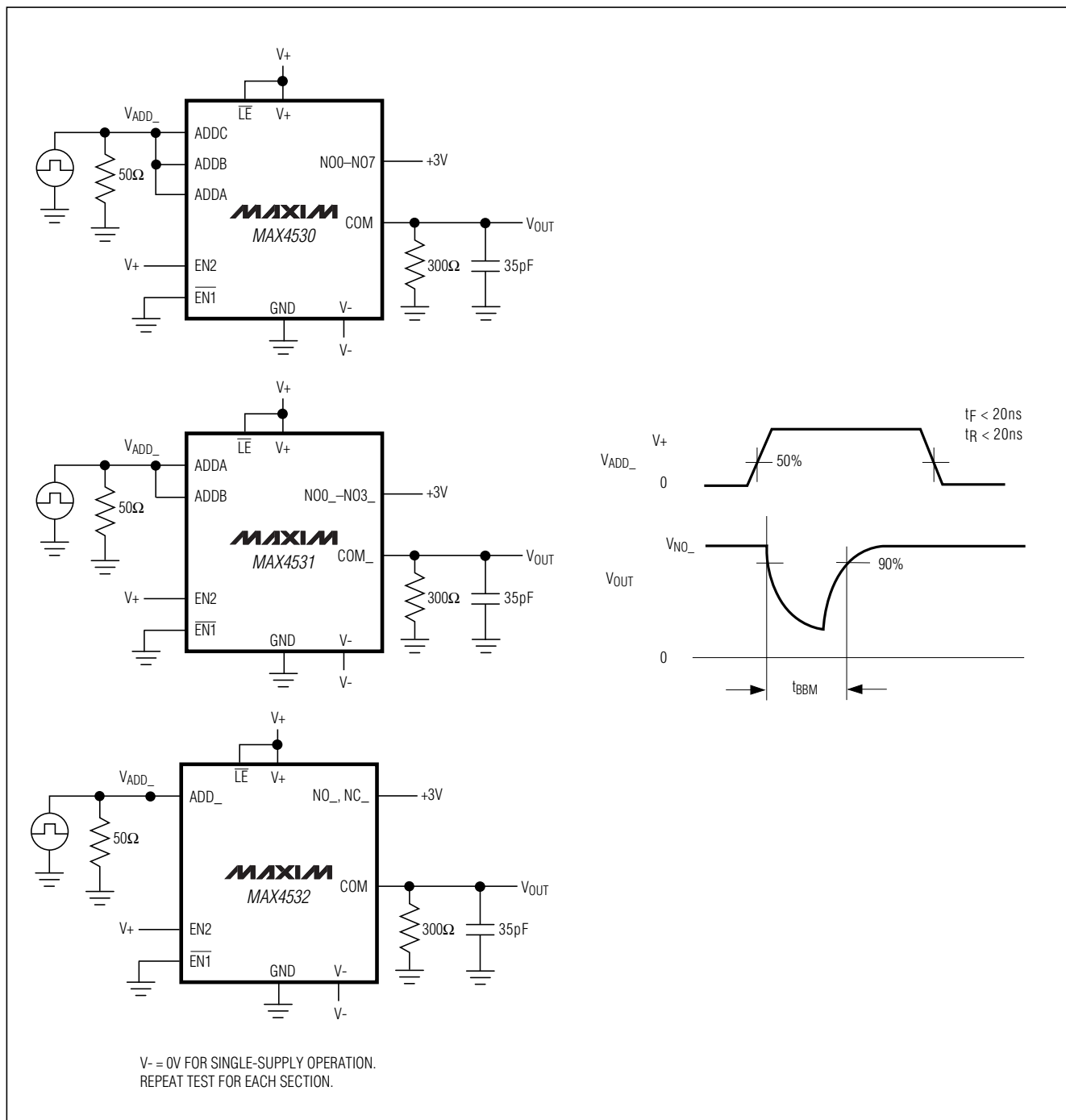
Figure 3. Break-Before-Make Interval
