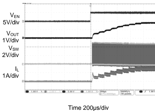
Enable Turn on ( I_{OUT} = 1.5A )
