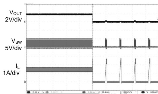
Short Circuit Protection ( I_{OUT} = 1.5A )
