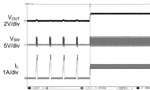
Short Circuit Protection Recovery ( I_{OUT} = 1.5A )
