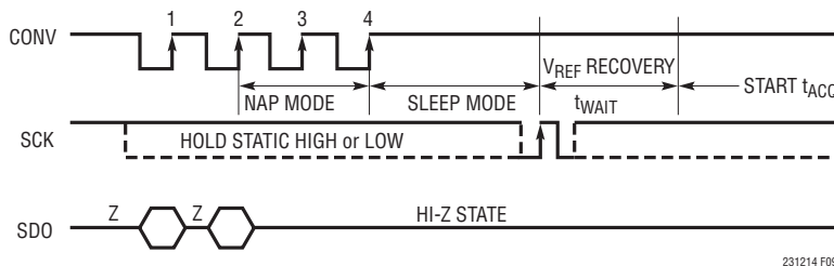
Figure 9. LTC2312-14 Entering/Exiting Sleep Mode
