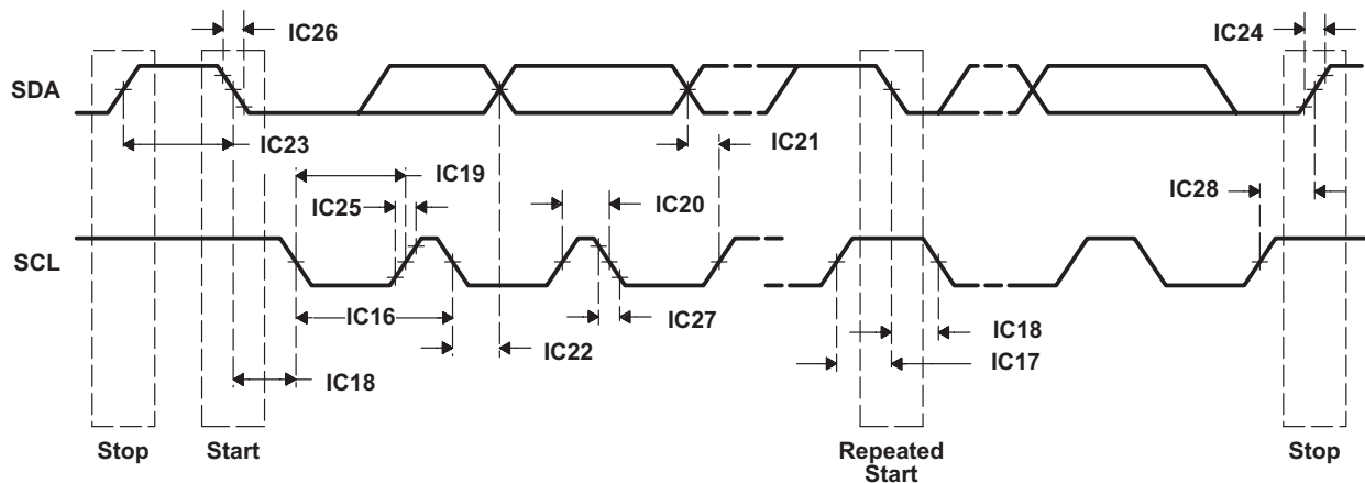
Figure 5-38. I²C Transmit Timings
