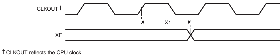
Figure 5-20. XF Timings
