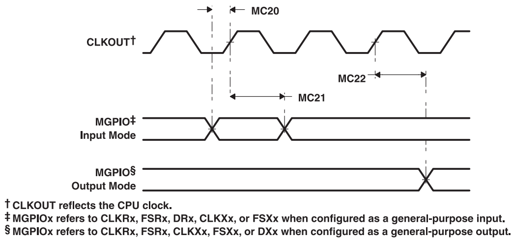
Figure 5-30. McBSP General-Purpose I/O Timings
