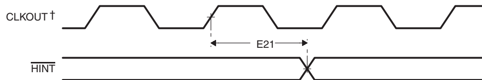
Figure 5-31. \overline{\text{HINT}} Timings
