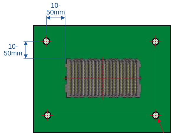
Recommended Spacer Location
