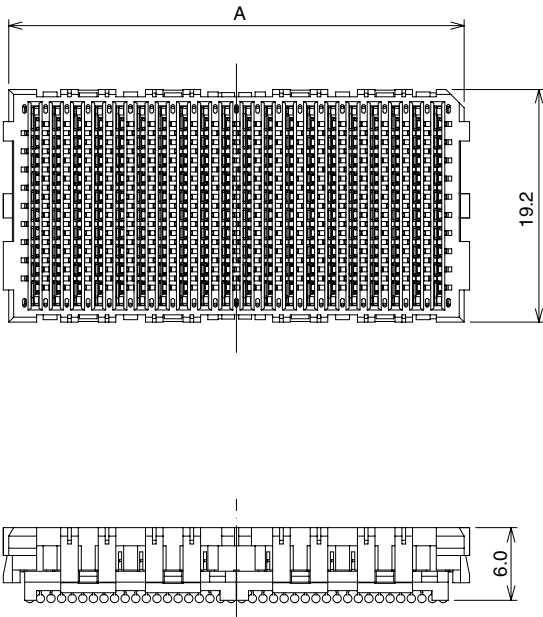
Shown: 200 position mating receptacle, IT3M-200S-BGA
