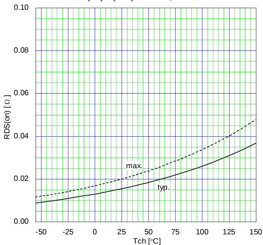
Drain-Source On-state Resistance R_{DS(on)}=f(T_{ch}):I_D=50\text{A}, V_{GS}=10\text{V}
