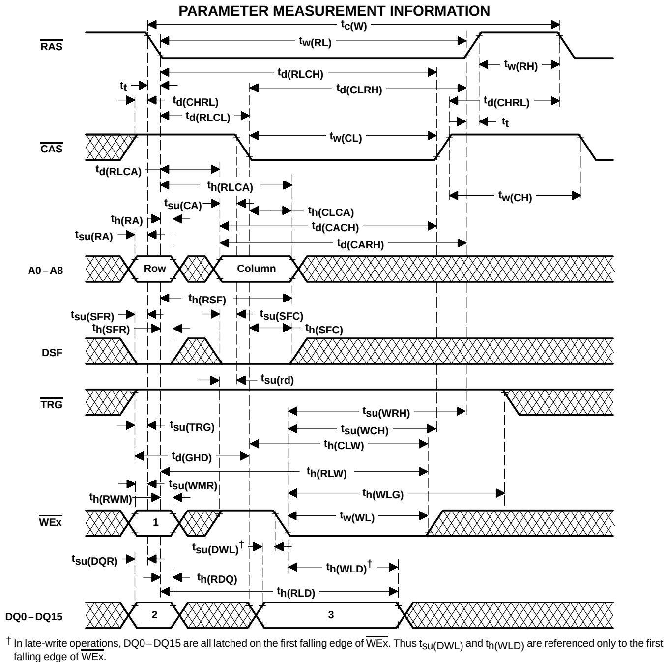
Figure 33. Late-Write-Cycle Timing (Output-Enable-Controlled Write)
