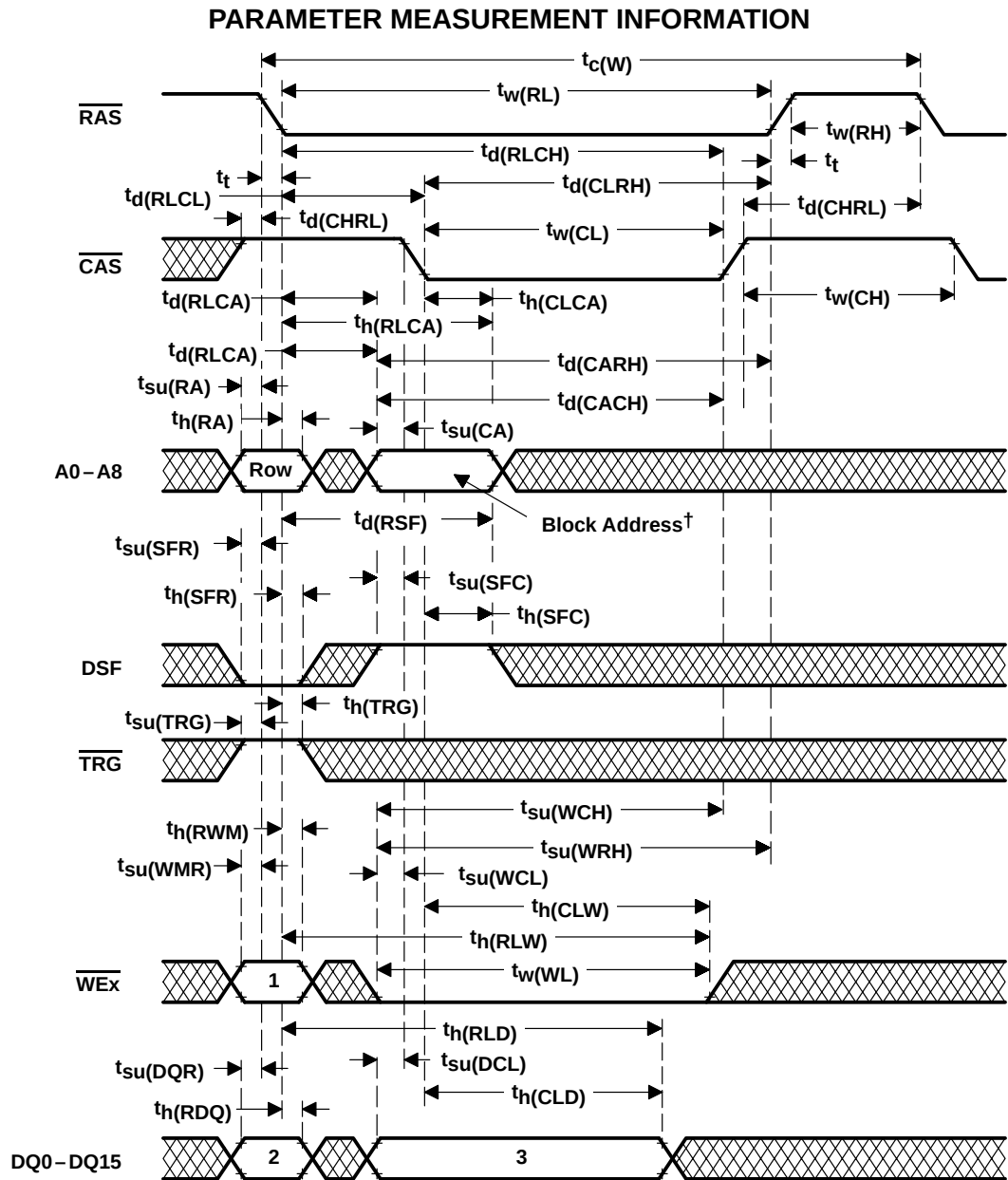
Figure 35. Block-Write-Cycle Timing (Early Write)
