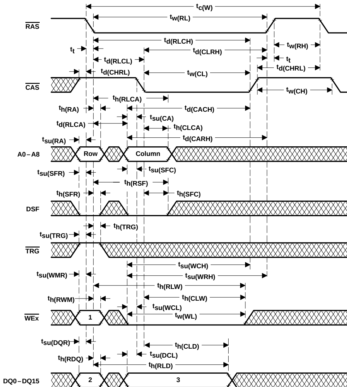
Figure 32. Early-Write-Cycle Timing
