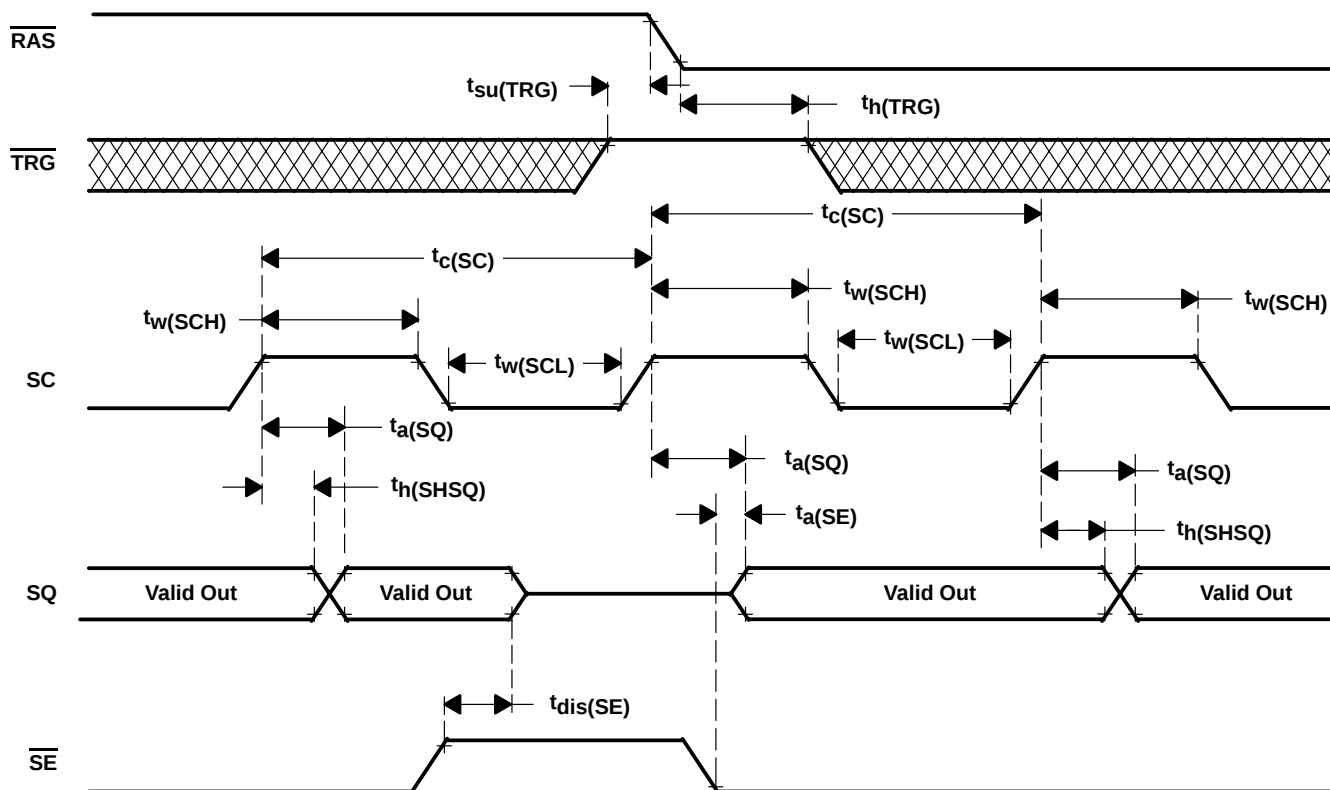
Figure 54. Serial-Read Timing ( \overline{\text{SE}} -Controlled Read)
