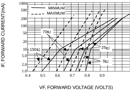
Fig. 10-TYPICAL FORWARD CHARACTERISTICS
