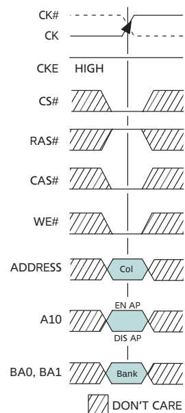
Figure 17: WRITE Command
