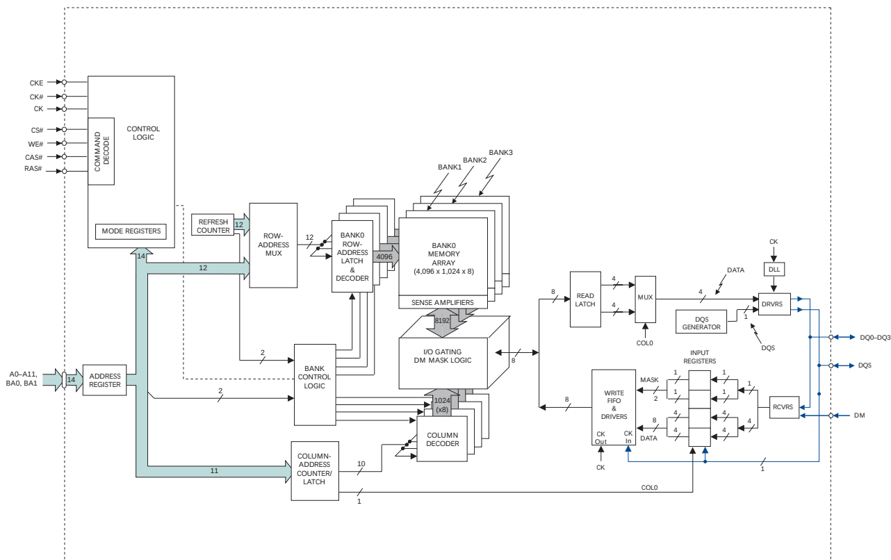
Figure 3: 32 Meg x 4 Functional Block Diagram
