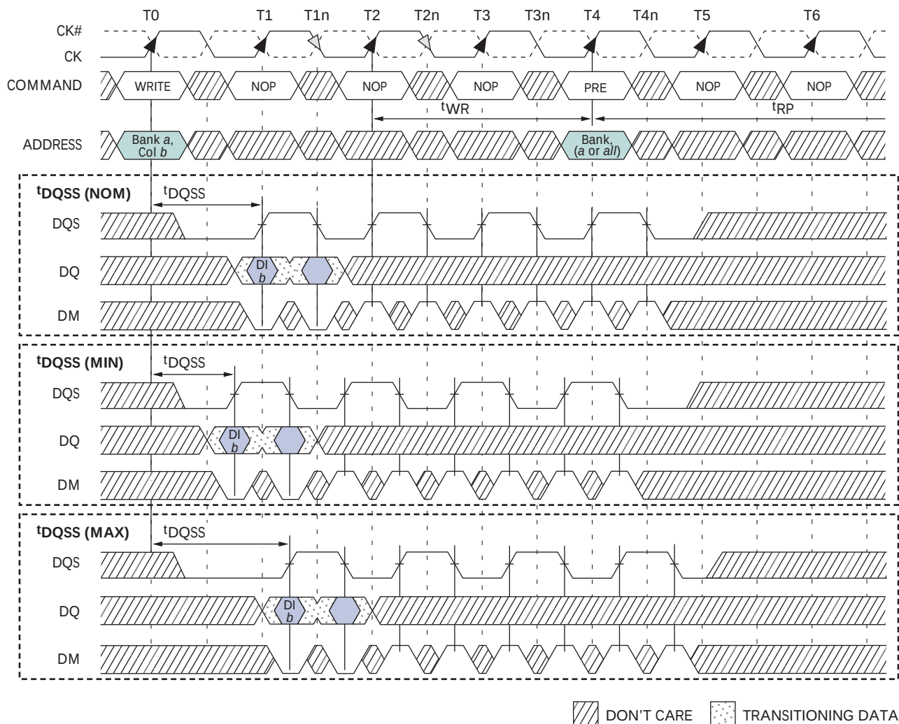
Figure 44: WRITE-to-PRECHARGE – Interrupting
