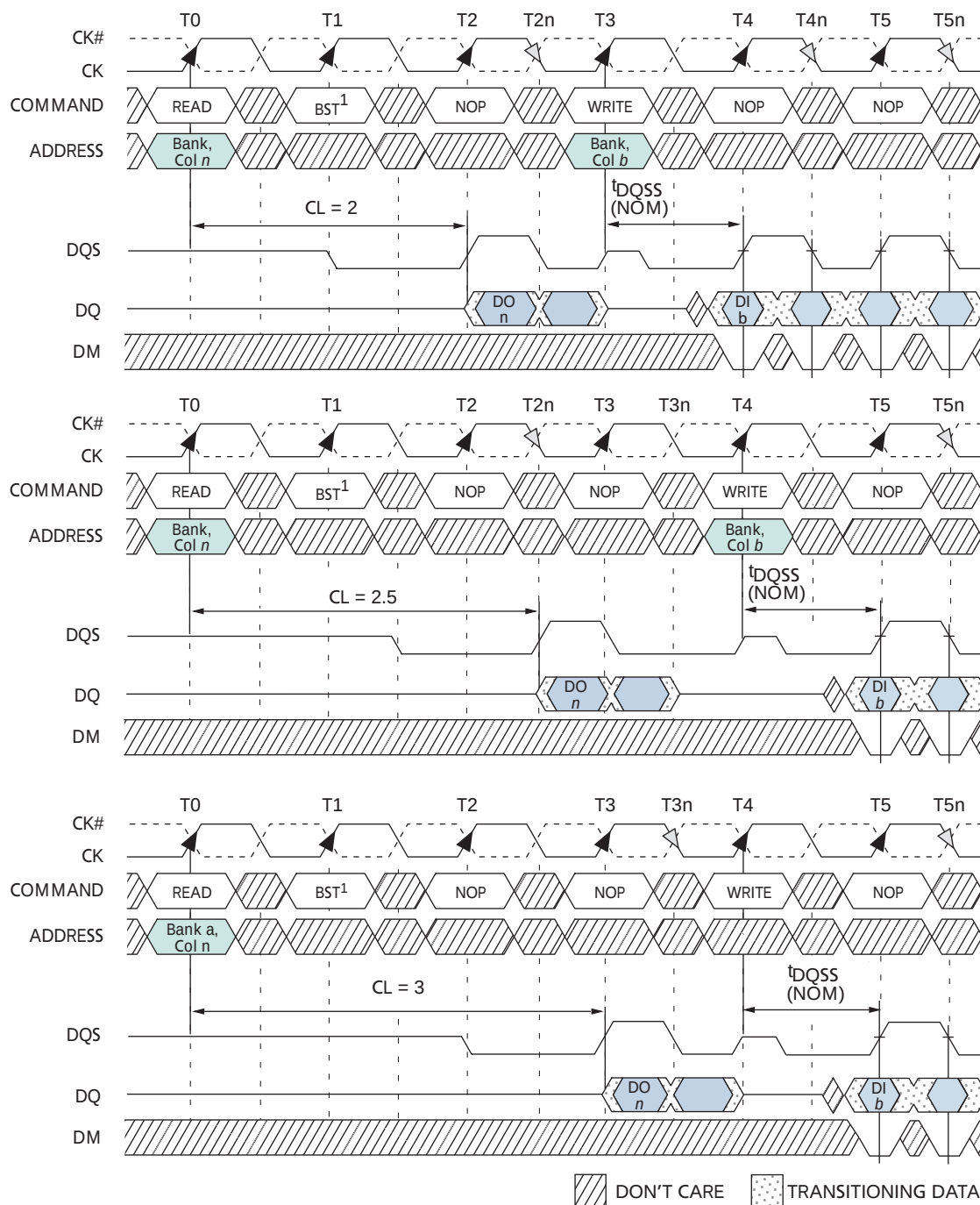
Figure 30: READ-to-WRITE
