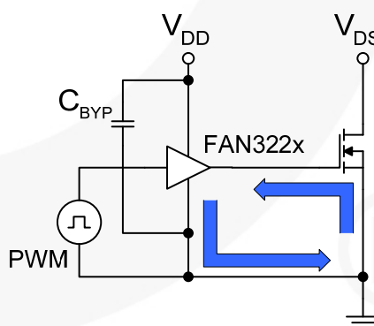
Figure 48. Current Path for MOSFET Turn-off
