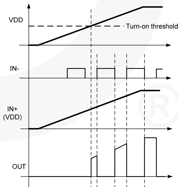
Figure 52. Inverting Start-Up Waveforms
