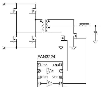
Figure 54. Center-tapped Bridge Output with Synchronous Rectifiers
