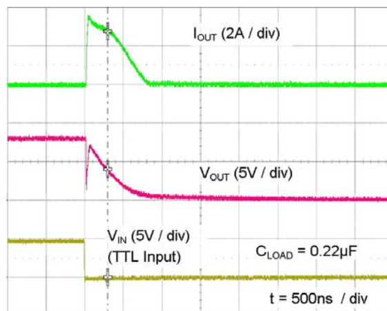
Figure 44. Quasi-Static Sink Current with V_{DD}=8V^{(14)}
