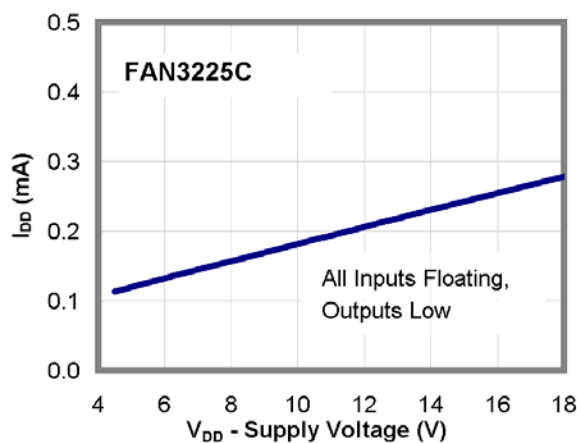
Figure 13. I_{DD} (Static) vs. Supply Voltage (13)
