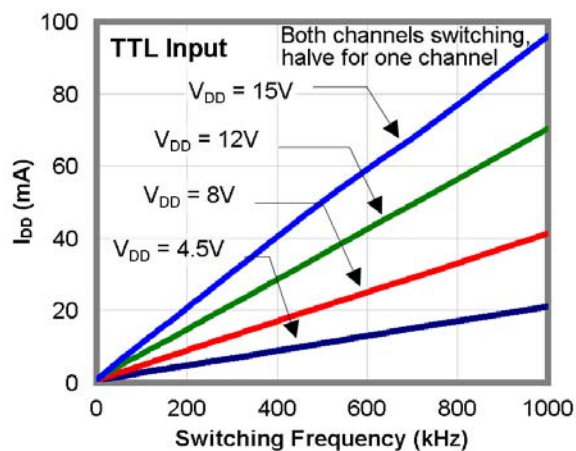
Figure 17. I_{DD} (2.2nF Load) vs. Frequency
