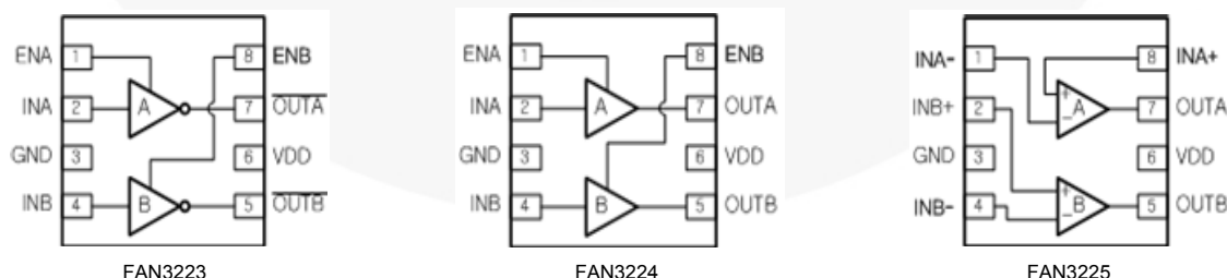
Figure 1. Pin Configurations
