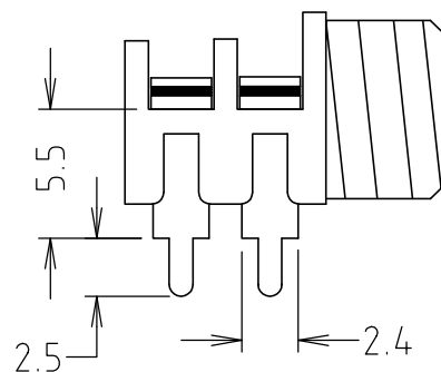
TYPE B 5.5mm CTR PCB
