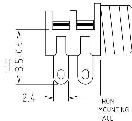
TYPE C SOLDER TAG
