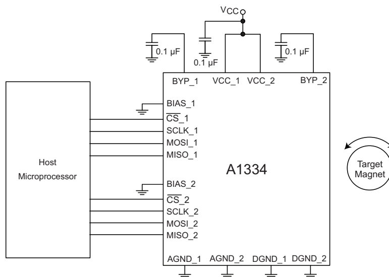
Either or both internal SoCs can be operated simultaneously. (See page 12 for circuits that require a higher level of EMC immunity.)
