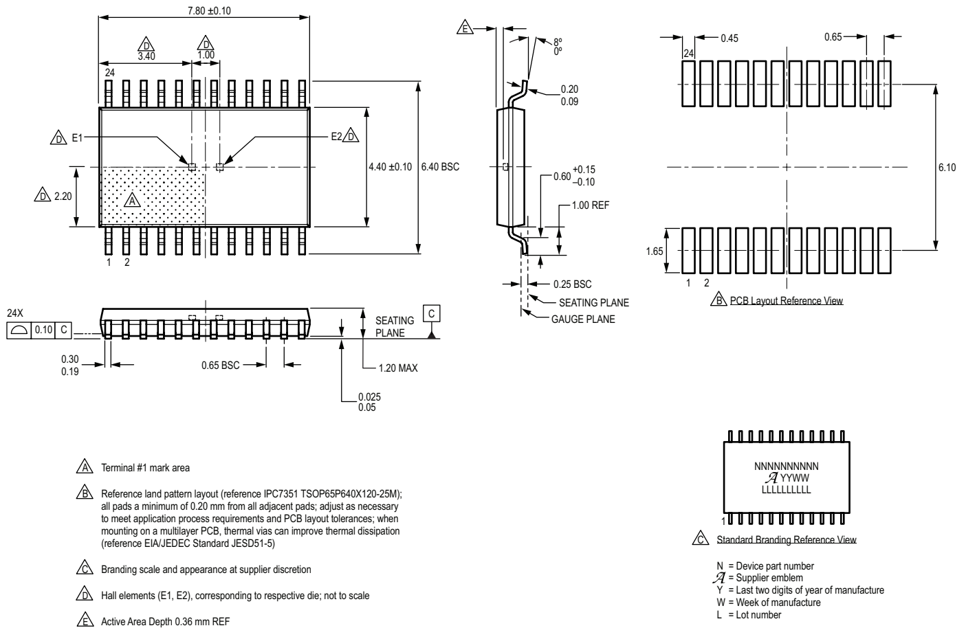
Figure 19: Package LE, 24-Pin TSSOP (Dual Die Version)
