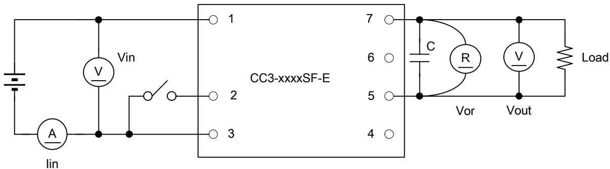
[5] Test Circuit
