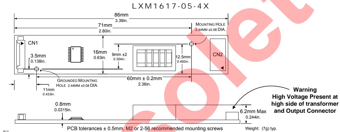
PHYSICAL DIMENSIONS
