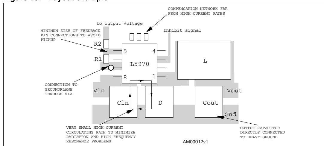
Figure 13. Layout example
