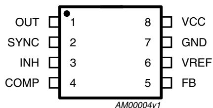
Figure 3. Pin connection
