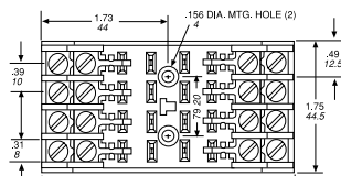
Cat. No. CR0002 With (#6) binding head screws
