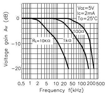
Fig. 10 Frequency Response
