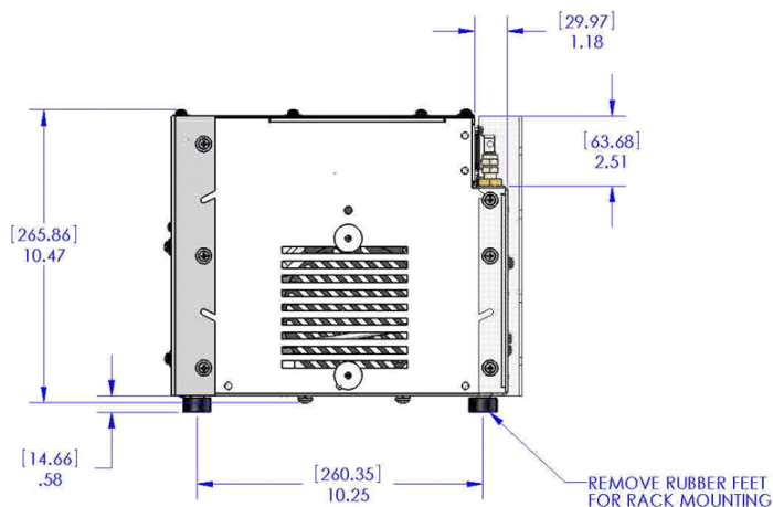
MT500B SIDE VIEW
