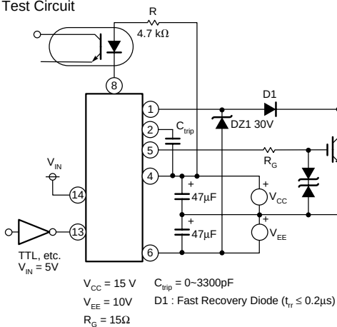
Test Circuit
