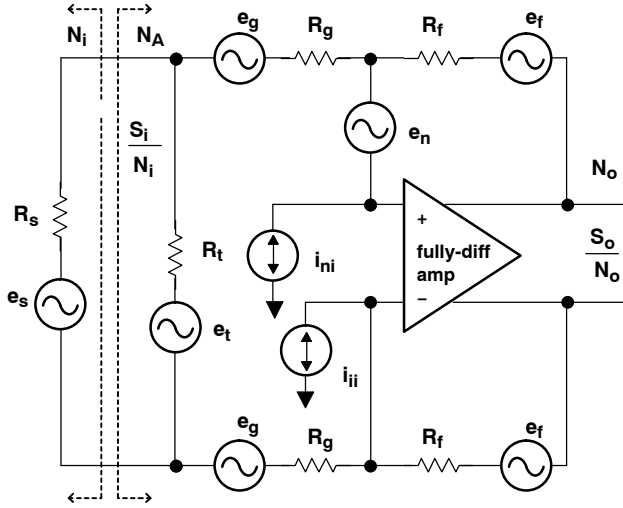
Figure 107. Noise Sources in a Fully Differential Amplifier Circuit
