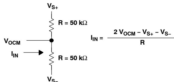
Equivalent Input Circuit for V_{OCM} Figure 102
