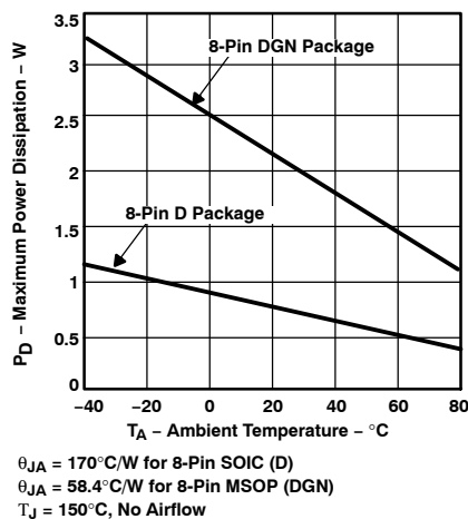
Figure 114. Maximum Power Dissipation vs Ambient Temperature
