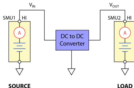
Figure 1: Circuit diagram showing a dual-channel SMU instrument in use for I/V characterization of a DC-DC converter.
