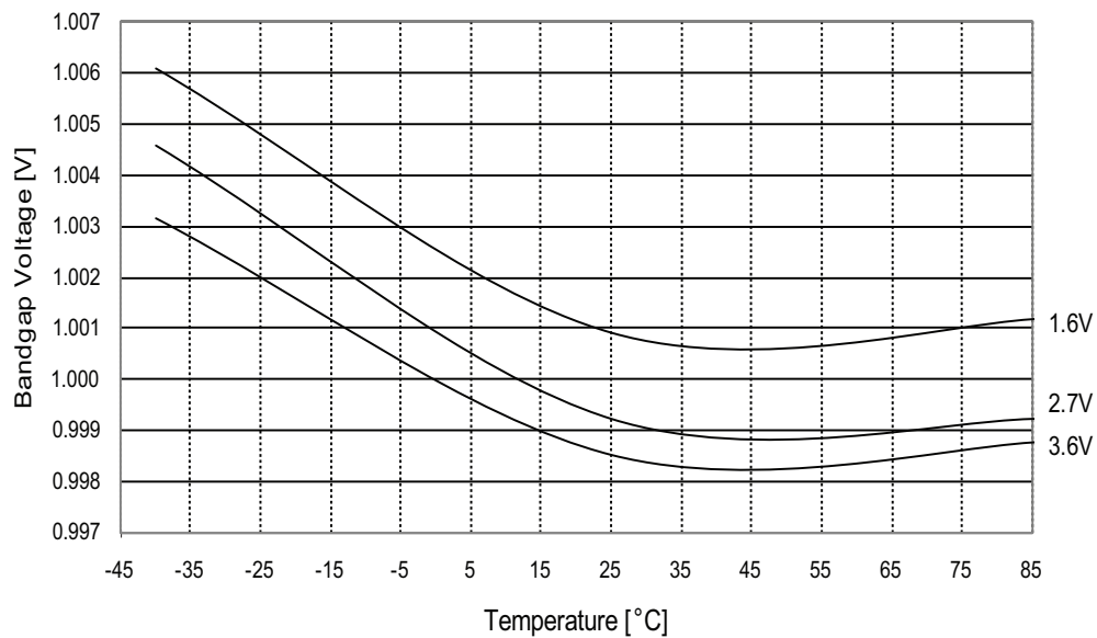
Figure 33-129. ADC internal 1.0V reference vs. temperature.
