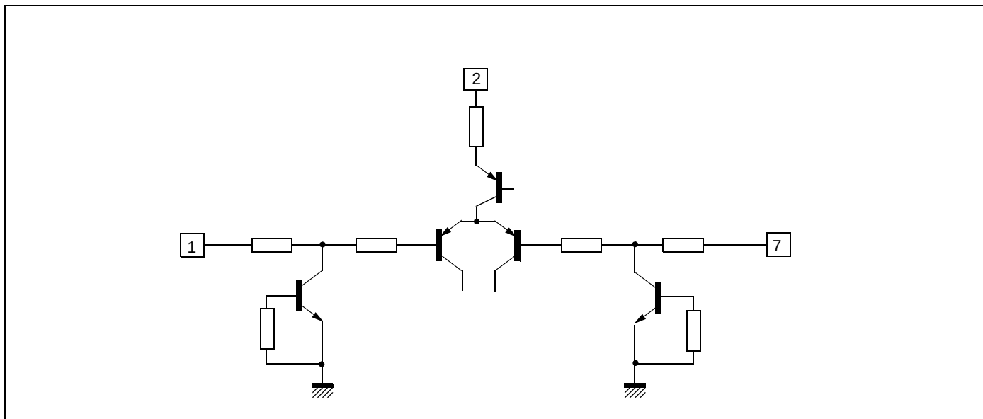
Figure 11: Pins 1 and 7
