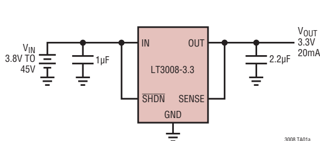
3.3V, 20mA Supply with Shutdown
