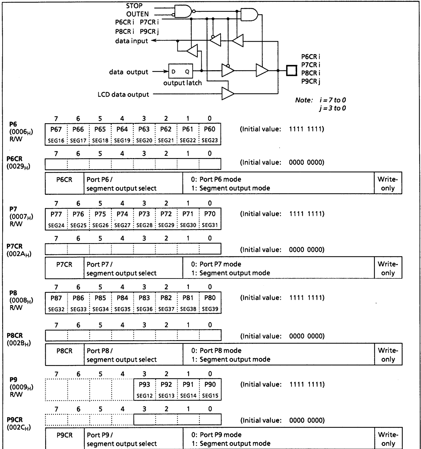
Figure 2-9. Port P6, P7, P8, P9
