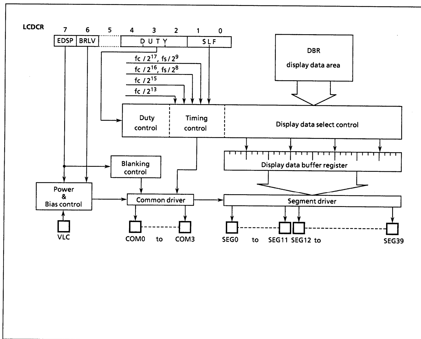
Figure 2-44. LCD driver
