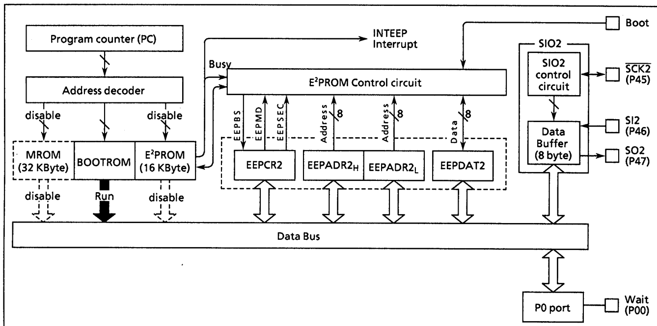
Figure 2-66. Program memory area of E 2 PROM (Serial PROM mode)
