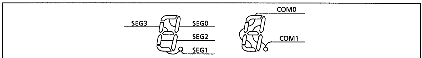
Figure 2-51. Example of COM, SEG Pin Connection
