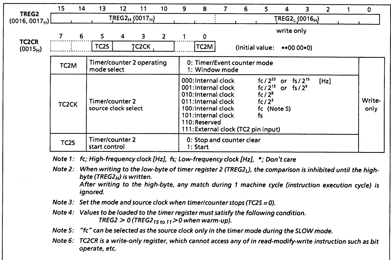
Figure 2-25. Timer Register 2 and TC2 Control Register
