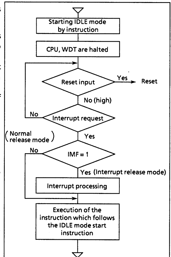
Figure 1-19. IDLE Mode
