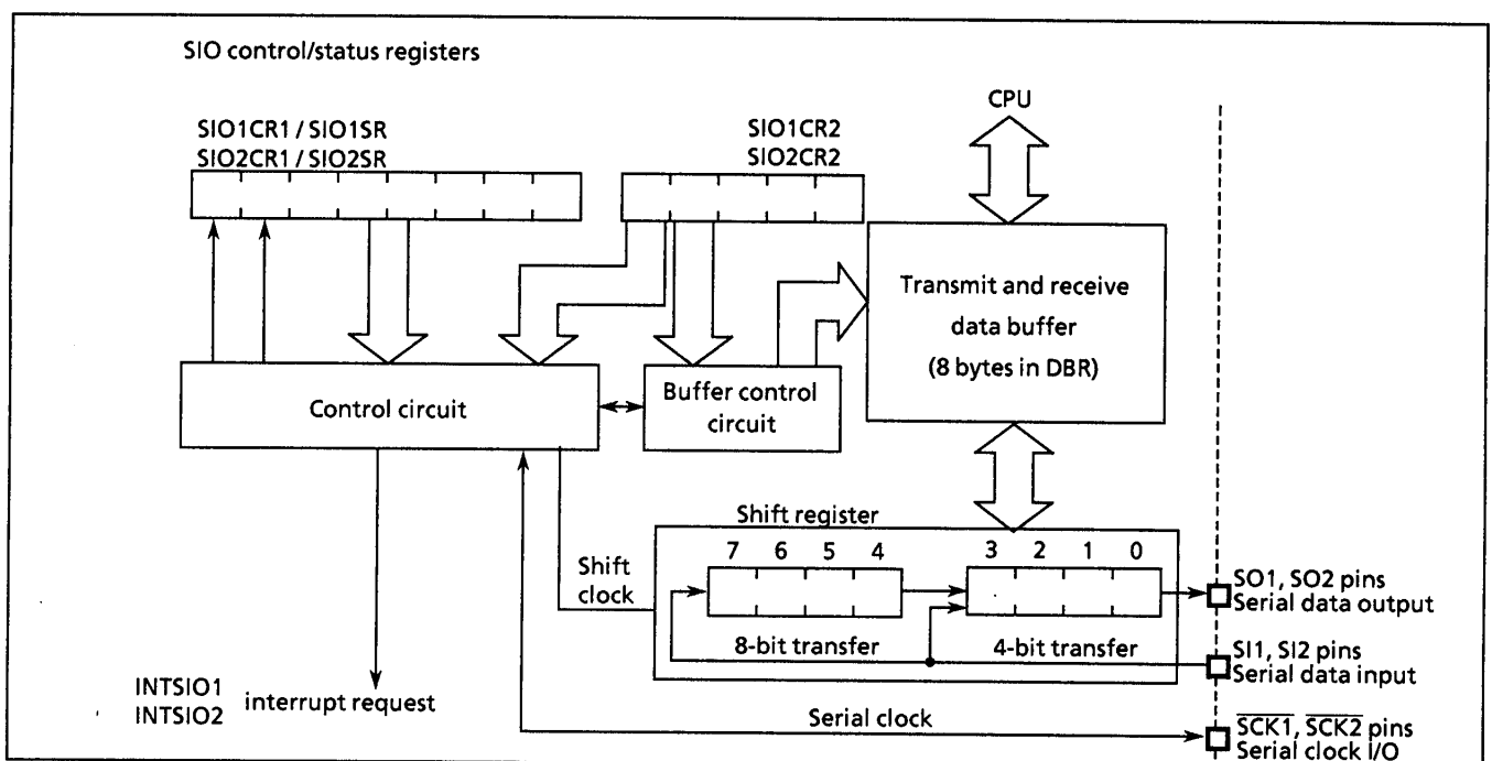
Figure 2-34. Serial Interfaces
