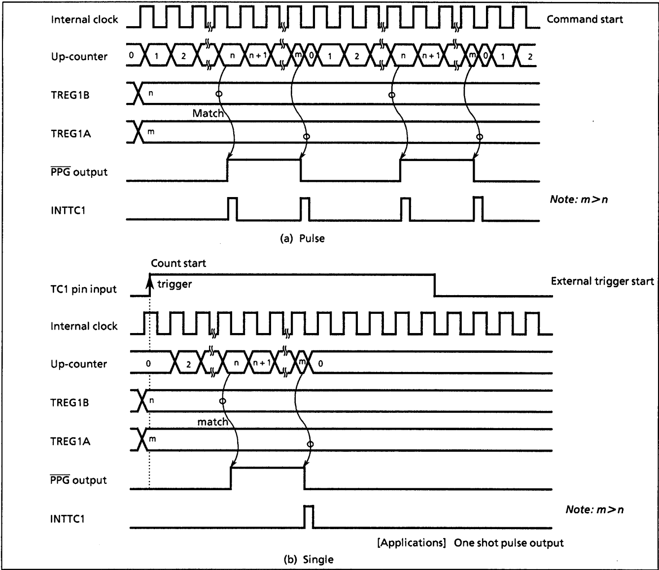
Figure 2-23. PPG Output Mode Timing Chart
