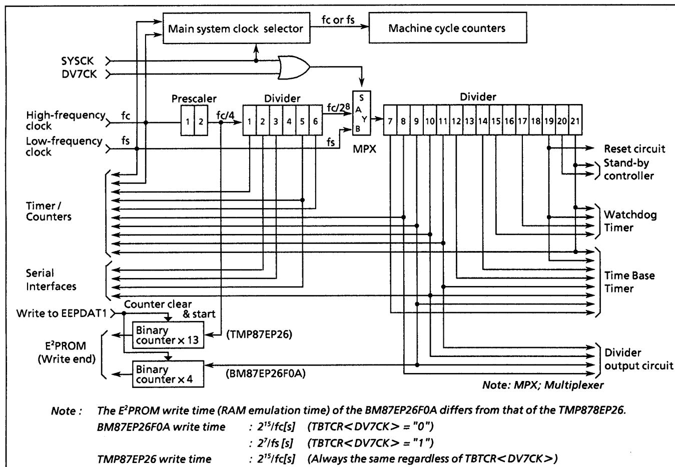
Figure 1-11. Configuration of Timing Generator
