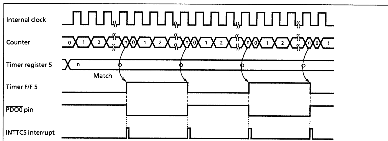
Figure 2-32. PDO Mode Timing Chart
