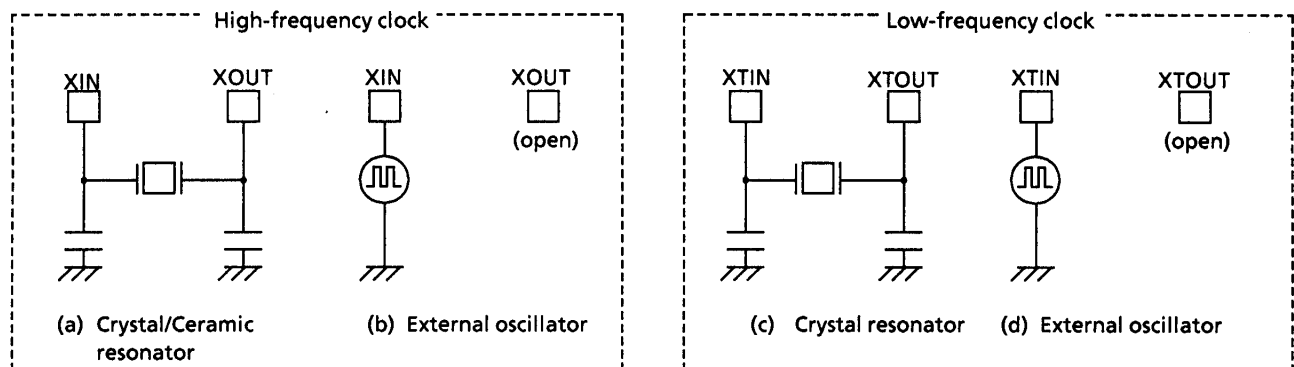
Figure 1-10. Examples of Resonator Connection
