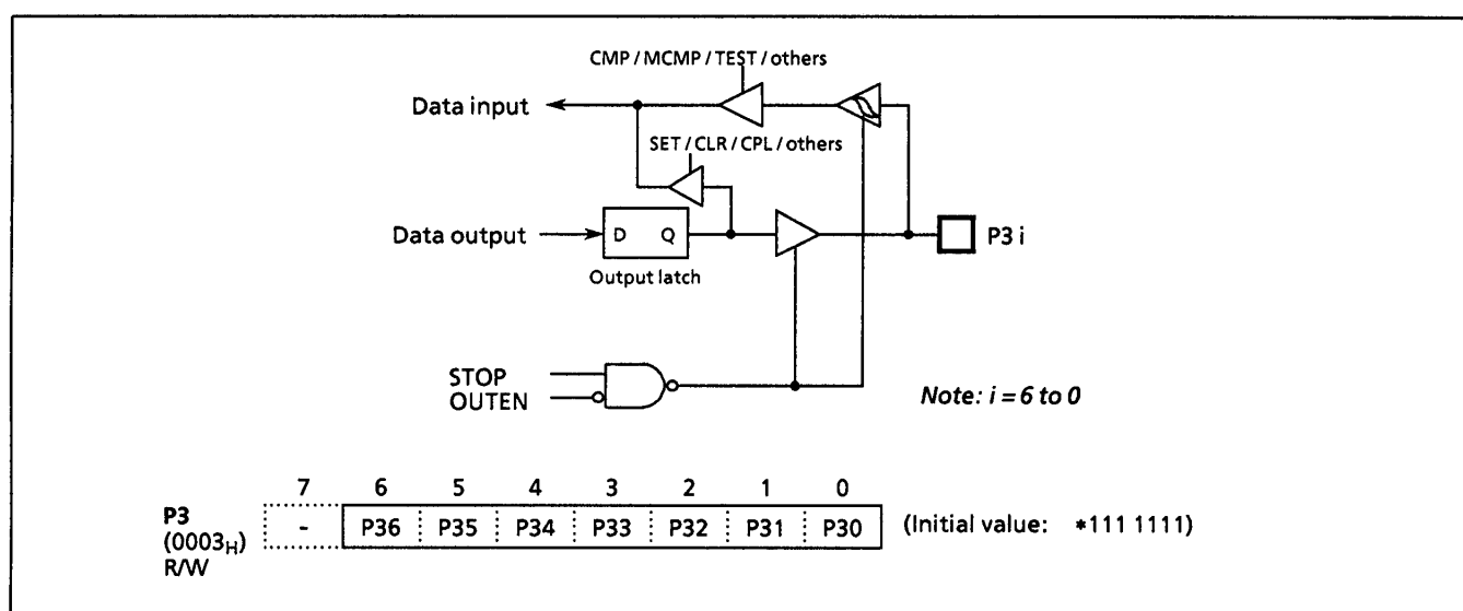
Figure 2-6. Port P3
