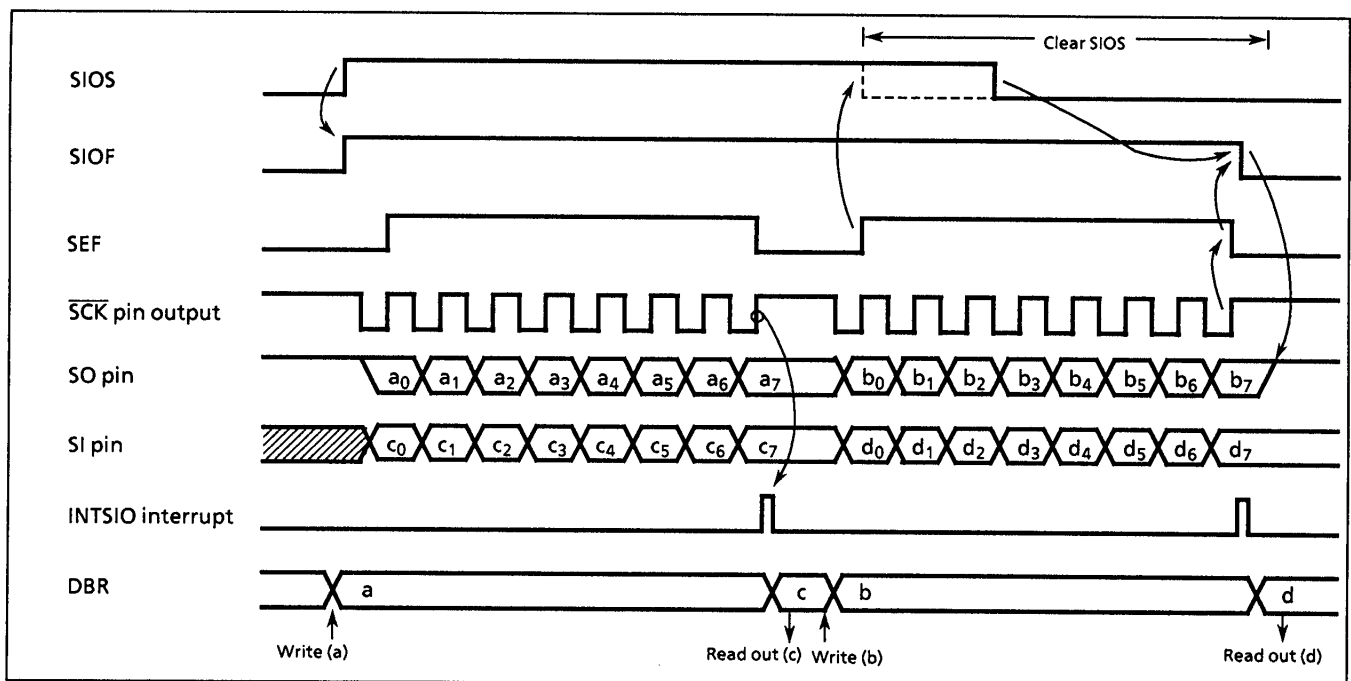
Figure 2-42. Transmit/Receive Mode (Example: 8-bit, 1word, internal clock)
