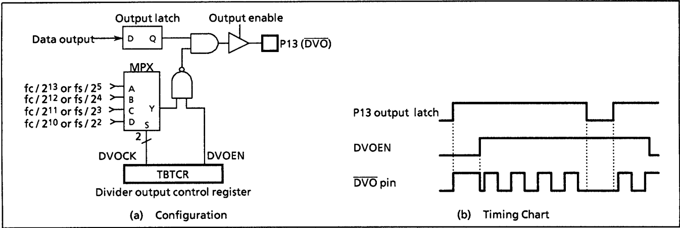
Figure 2-14. Divider Output
