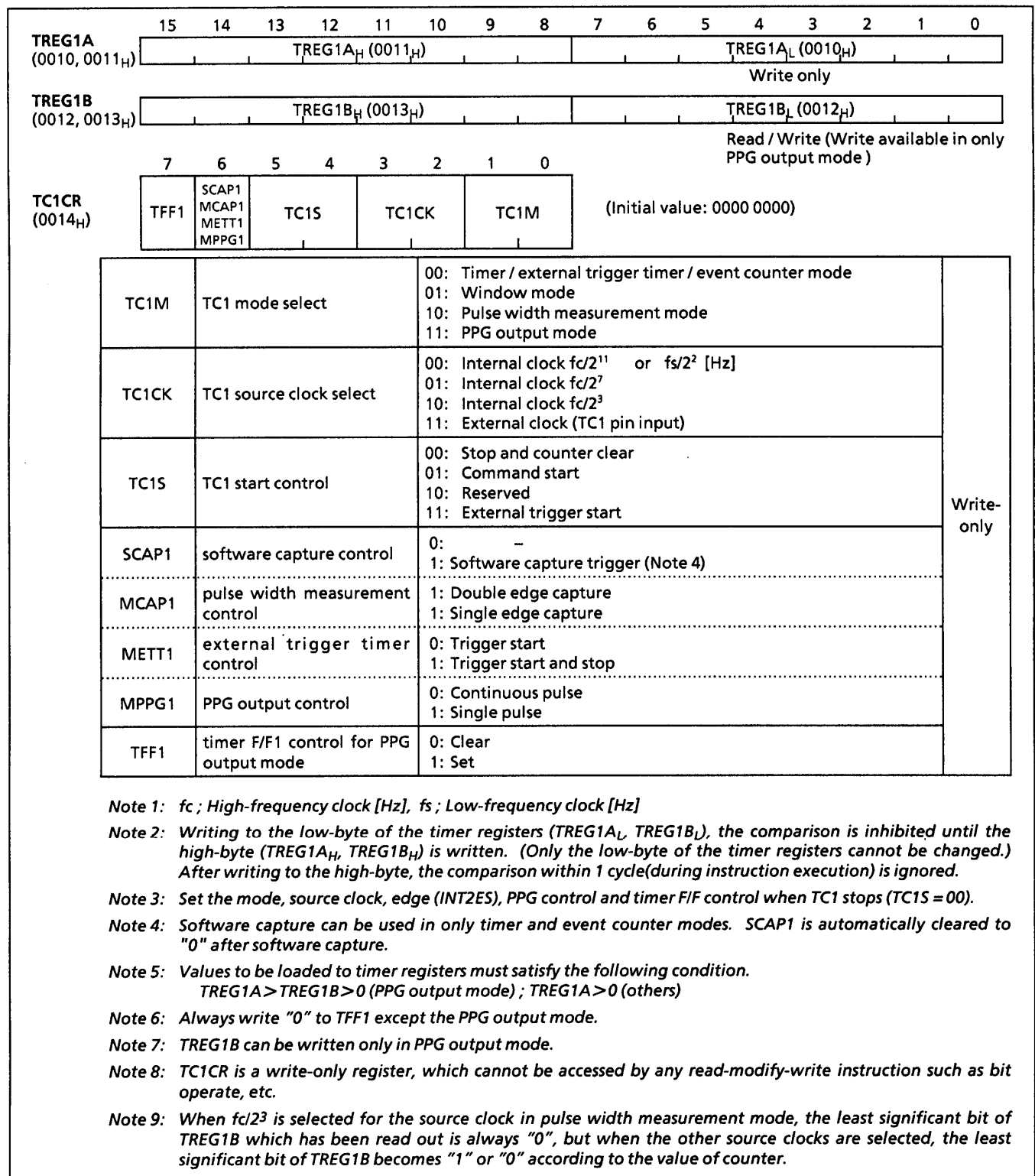
Figure 2-16. Timer Registers and TC1 Control Register
