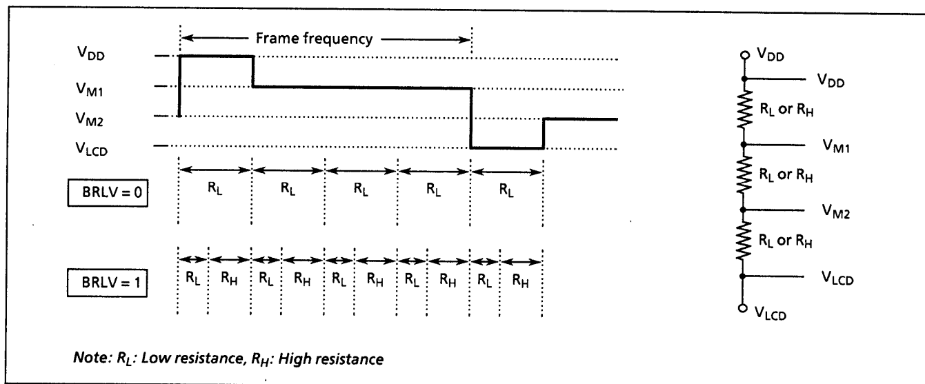
Figure 2-46. Selecting split resistance with BRLV setting (1/3 bias)
