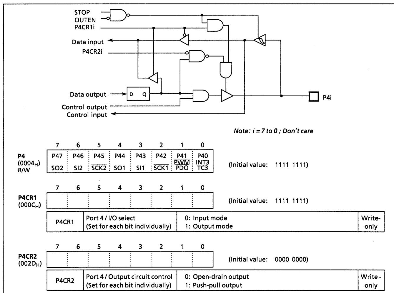
Figure 2-7. Port P4
