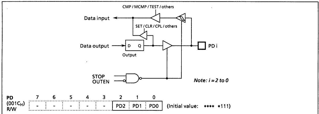
Figure 2-10. Port PD
