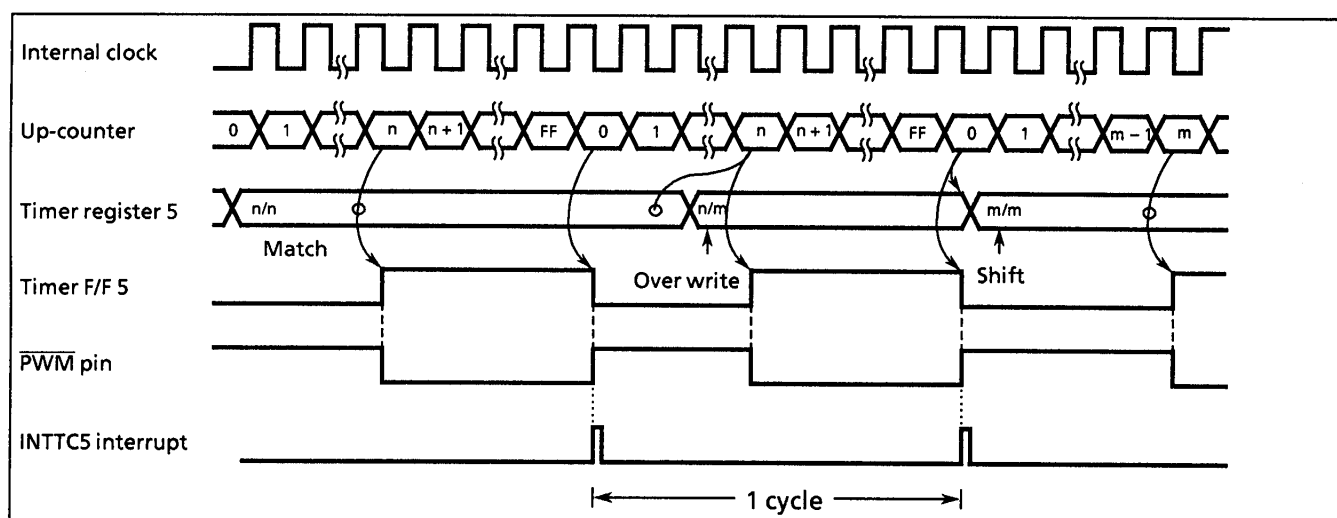
Figure 2-33. PWM Output Mode Timing Chart
