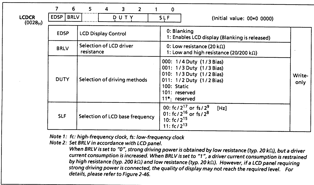
Figure 2-45. LCD driver control register
