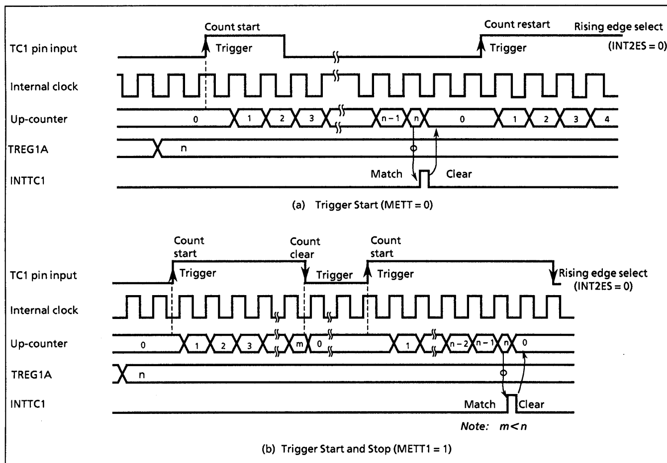
Figure 2-18. External Trigger Timer Mode Timing Chart
