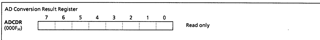
Figure 2-58. AD converter Result Register
