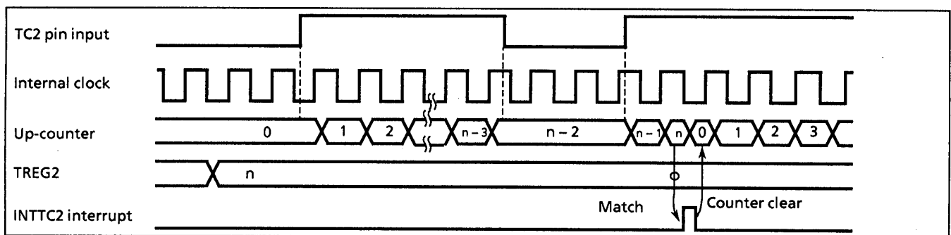
Figure 2-26. Window Mode Timing Chart
