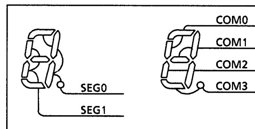
Figure 2-50. Example of COM, SEG Pin Connection (1/4 Duty)
