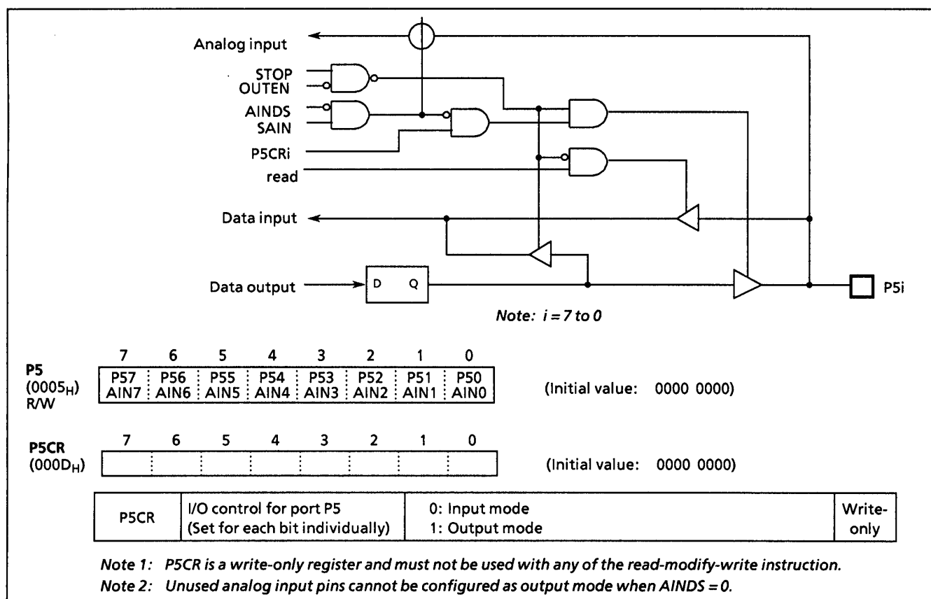
Figure 2-8. Port P5
