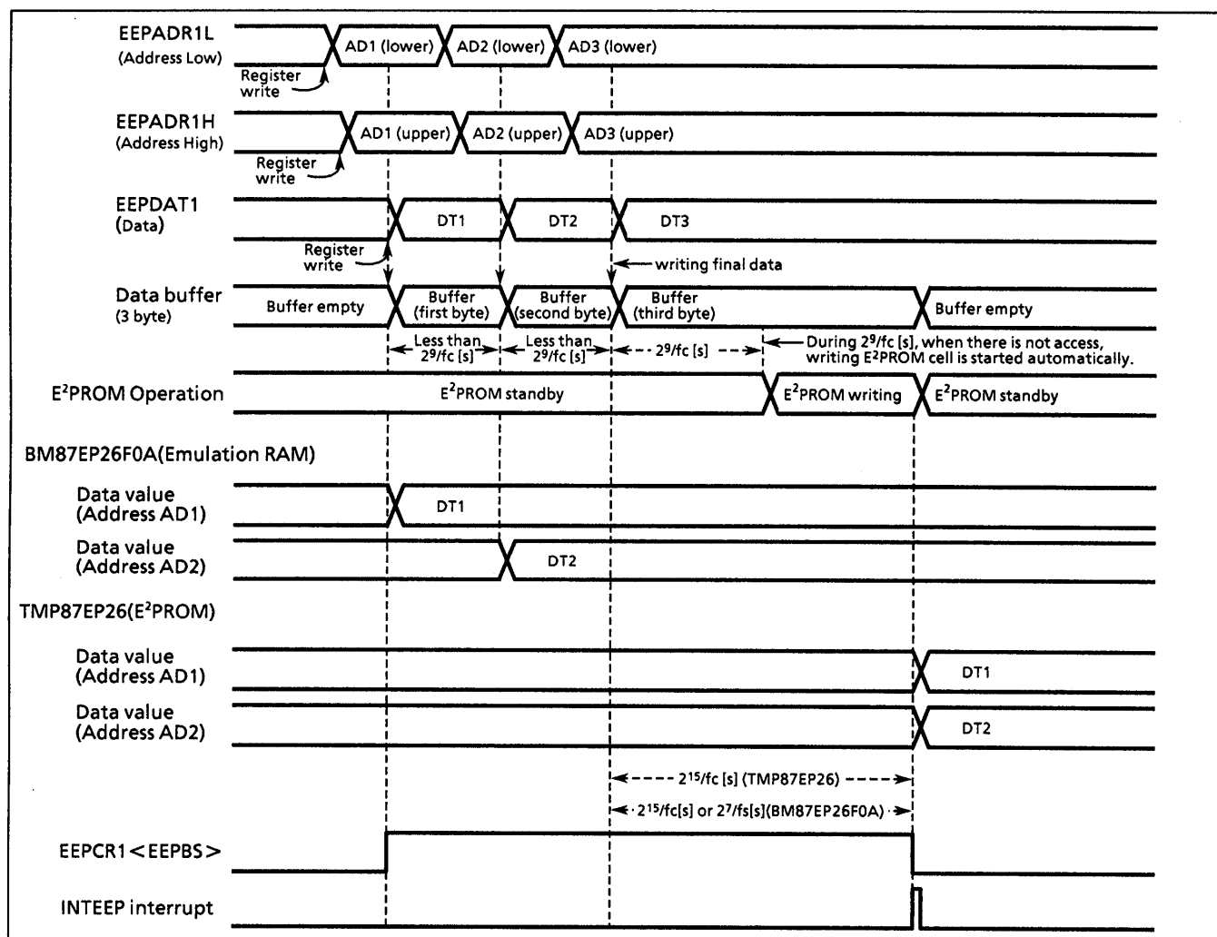
Figure 2-65. Write timing of BM87EP26F0A and TMP87EP26 (In case of 3 byte transfer)
