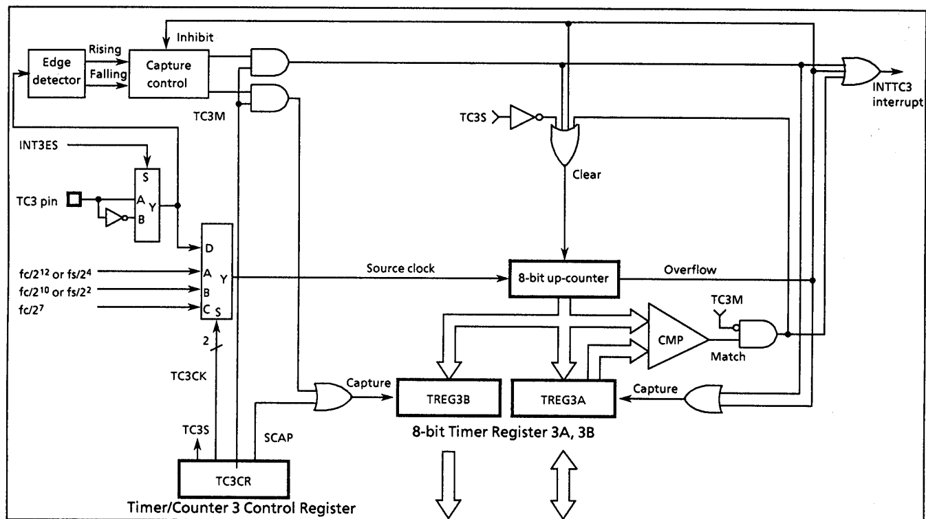
Figure 2-27. Timer/Counter 3
