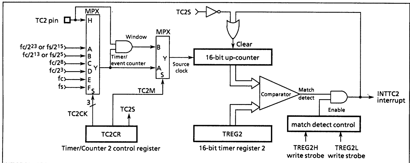
Figure 2-24. Timer/Counter 2 (TC2)
