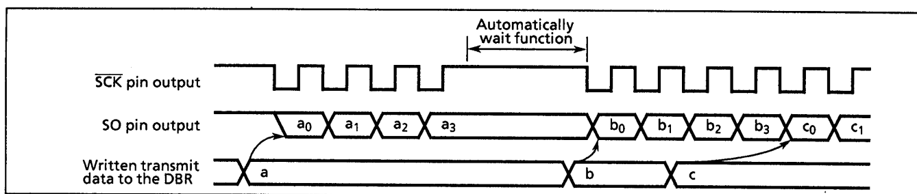
Figure 2-36. Clock Source (Internal Clock)
