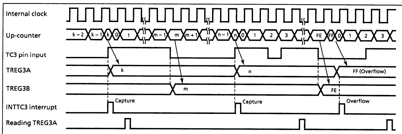
Figure 2-29. Timing Chart for Capture Mode (INT3ES = 0)
