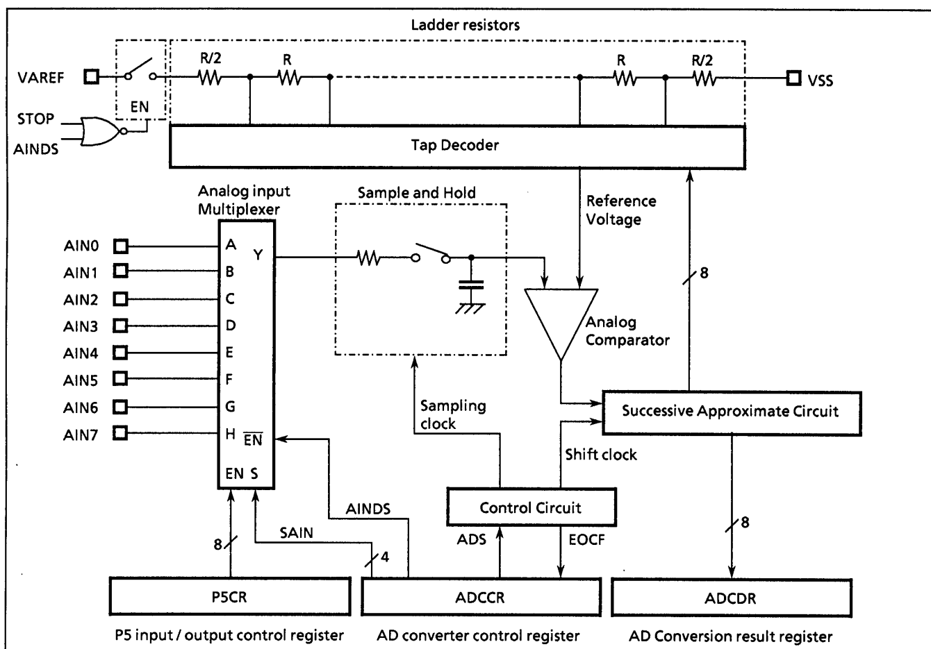
Figure 2-57. AD converter
