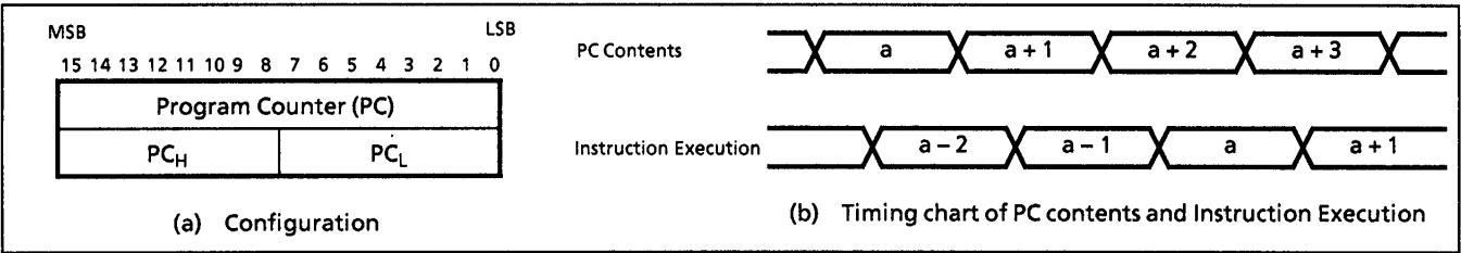
Figure 1-3. Program Counter
