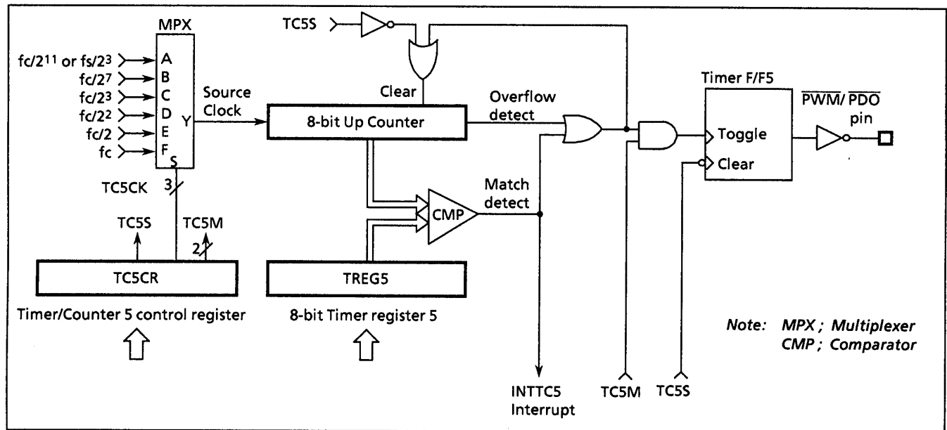
Figure 2-30. Timer/Counter 5 (TC5)
