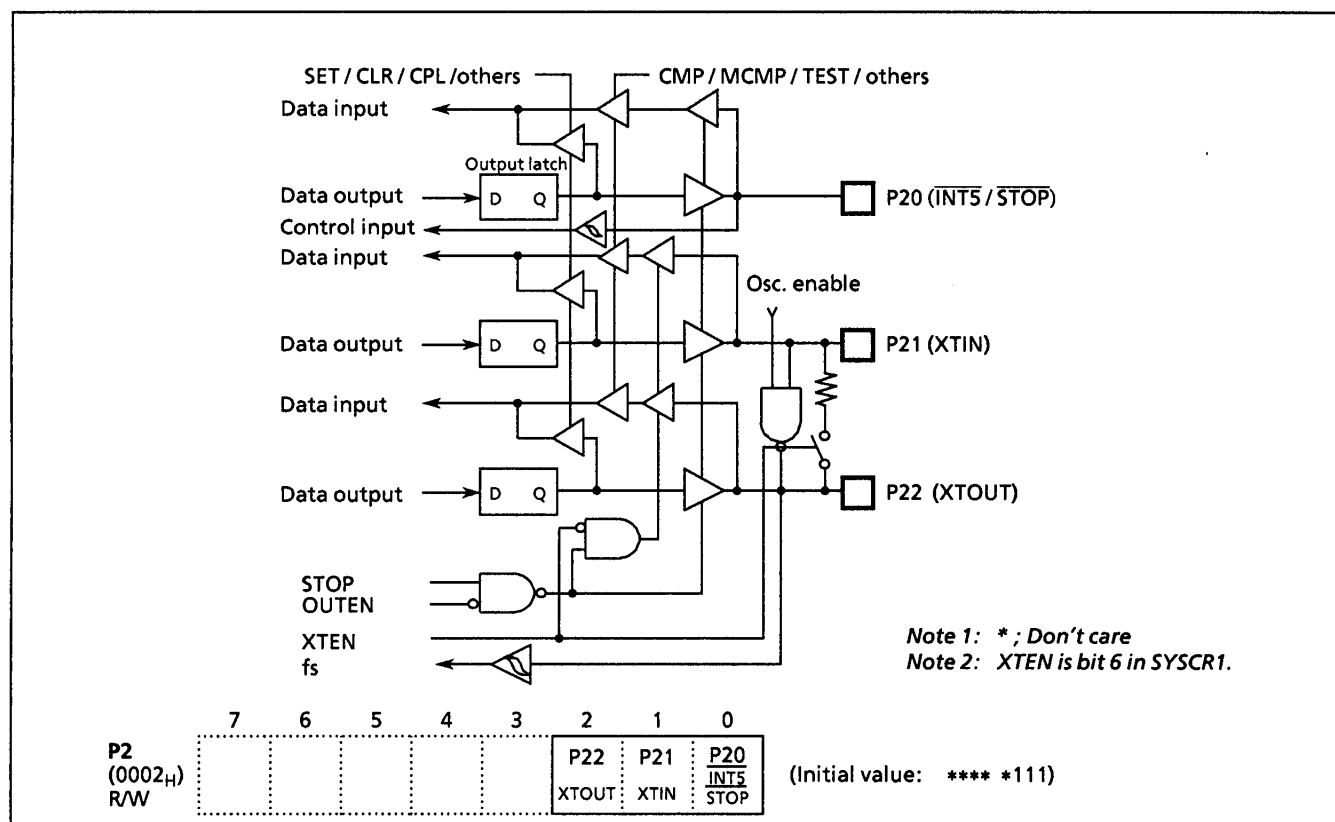
Figure 2-5. Port P2
