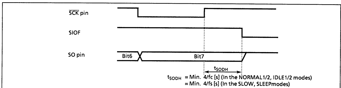
Figure 2-43. Transmitted Data Hold Time at end of transmit/receive
