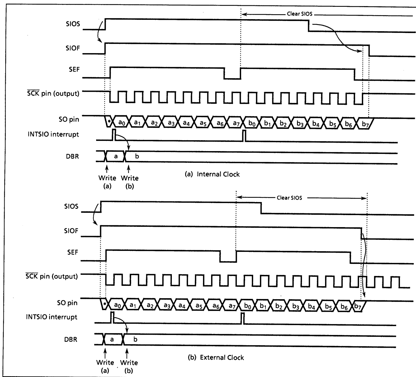
Figure 2-39. Transfer Mode (Example: 8-bit, 1 Word Transfer)
