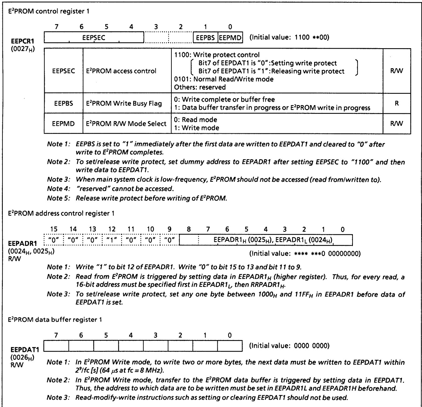
Figure 2-63. E 2 PROM control registers (Data memory)
