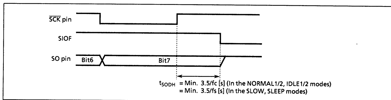
Figure 2-40. Transmitted Data Hold Time at end of transmit
