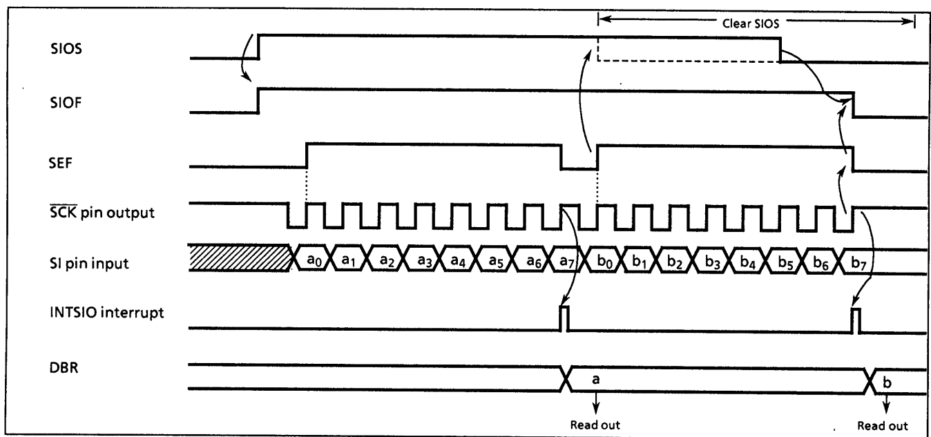
Figure 2-41. Receive Mode (Example: 8-bit, 1 word, internal clock)
