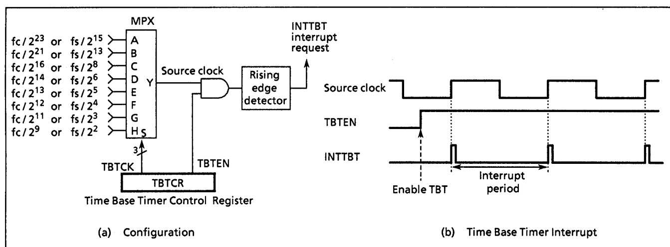
Figure 2-11. Time Base Timer
