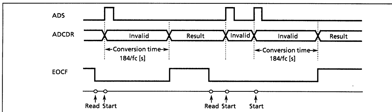
Figure 2-60. AD conversion Timing chart
