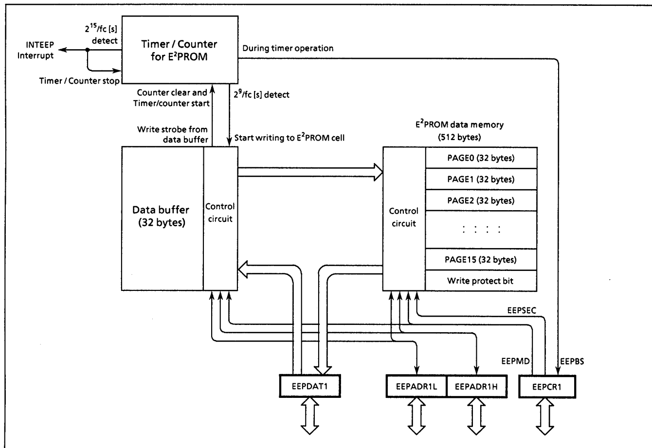
Figure 2-62. E 2 PROM Data Memory
