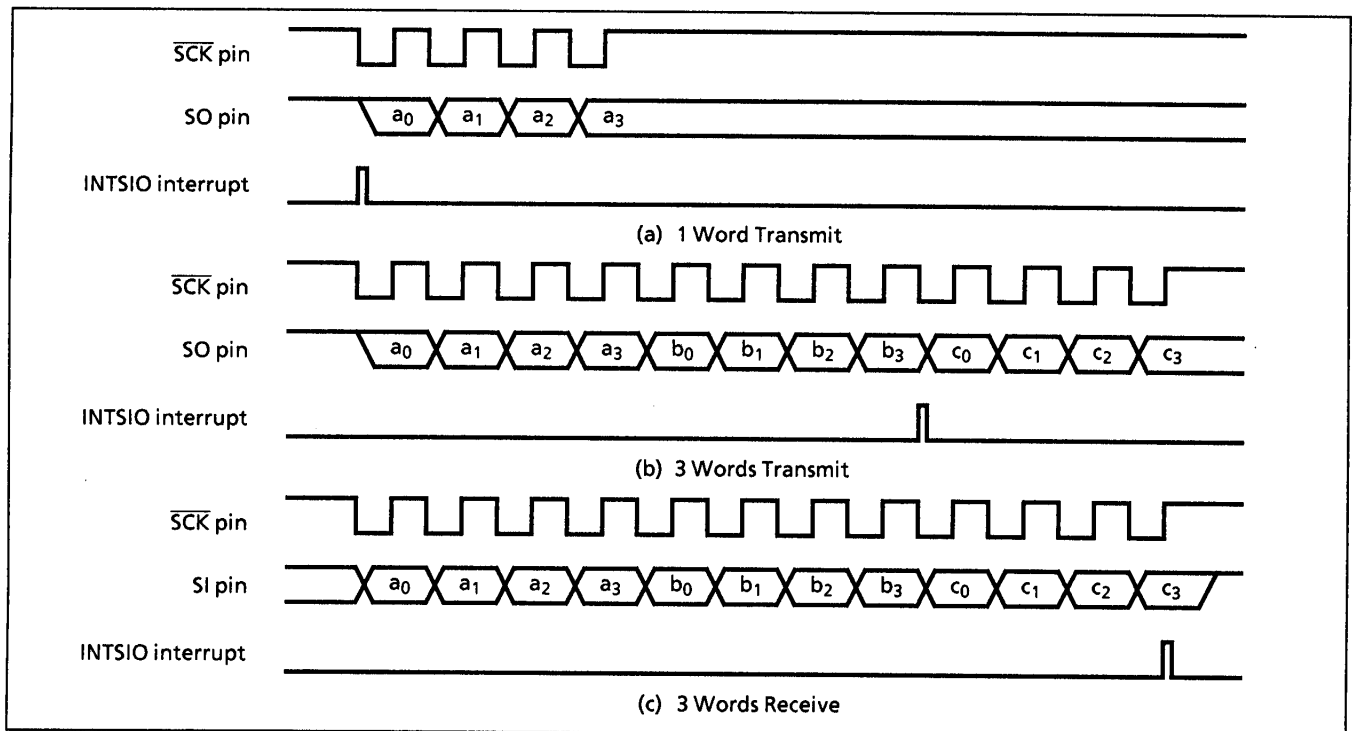
Figure 2-38. Number of Bits to Transfer (Example: 4-bit serial transfer)
