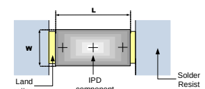
(0402 PCB footprint)
