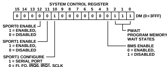
Figure 7. System Control Register
