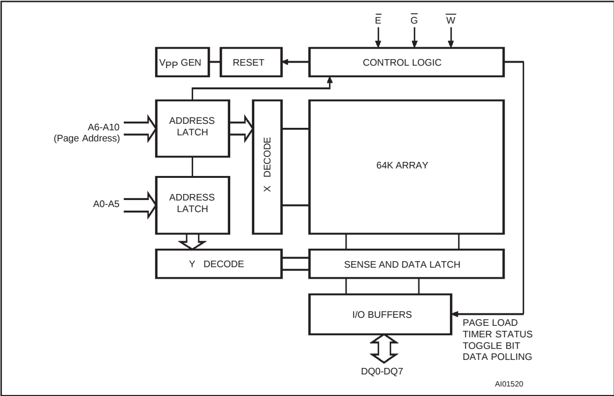
Figure 3. Block Diagram
