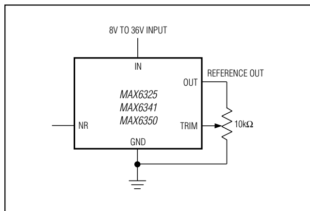
Figure 1. Output Voltage Adjustment
