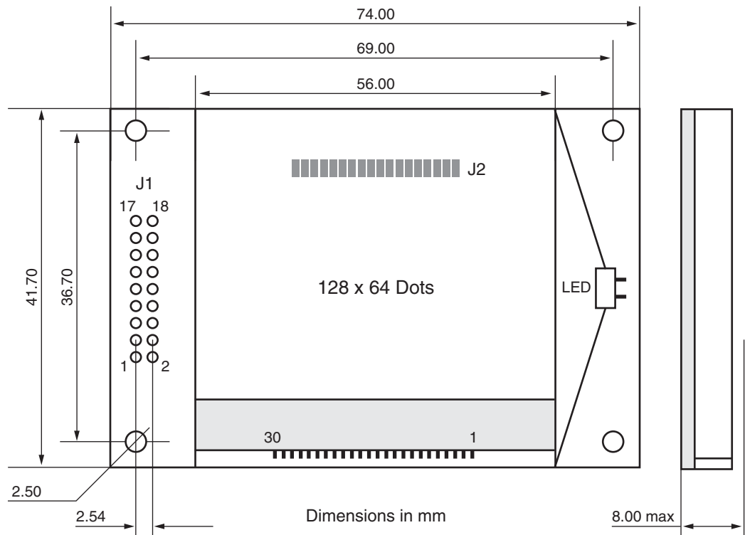
Figure 3-5: 64128EFCBC-3LP Dimensions
