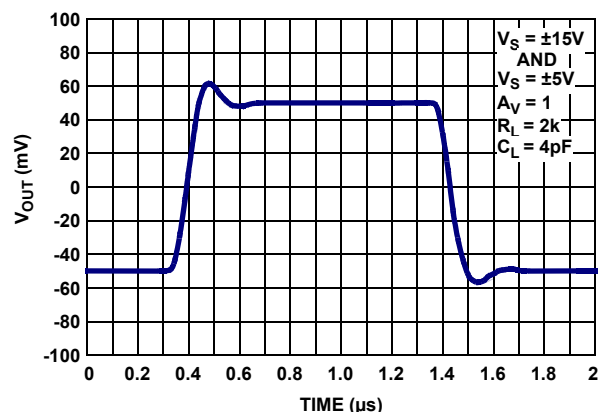
FIGURE 48. SMALL SIGNAL TRANSIENT RESPONSE, V_S = \pm 5V, \pm 15V
