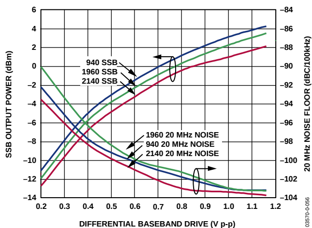
Figure 56. SSB P_{OUT} and 20 MHz Noise Floor vs. Baseband Drive Level ( F_{LO} = 940 \text{ MHz}, 1960 \text{ MHz}, \text{ and } 2140 \text{ MHz} )
