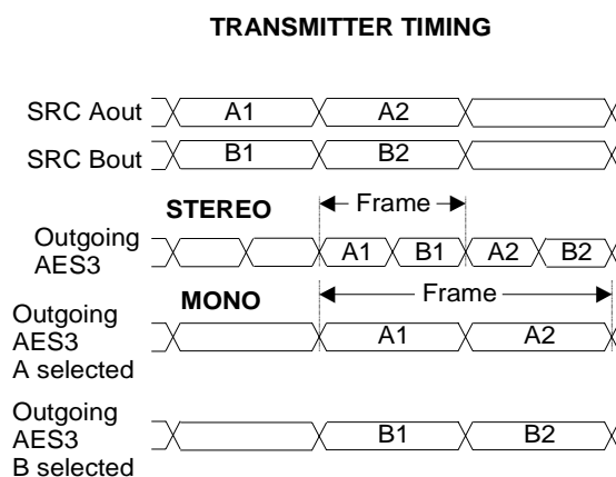
Figure 23. Mono Mode Operation Compared to Normal Stereo Operation
