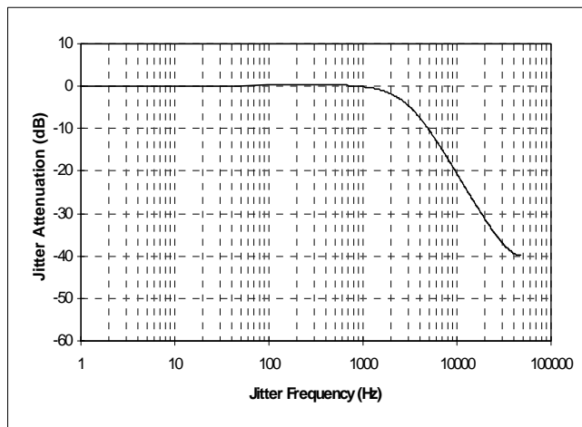
Figure 19. Jitter Attenuation Characteristics of PLL with “medium” Filter Components
