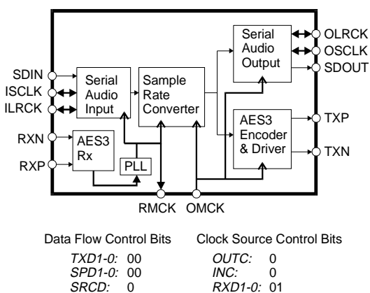
Figure 10. Serial Audio Input, AES3 Input Clock
