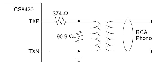
Figure 33. Consumer Output Circuit
