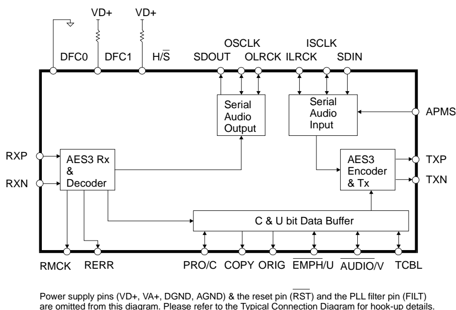
Figure 29. Hardware Mode 4 - Transceive Data Flow, without SRC
