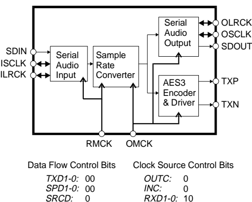
Figure 8. Serial Audio Input, No PLL, SRC enabled
