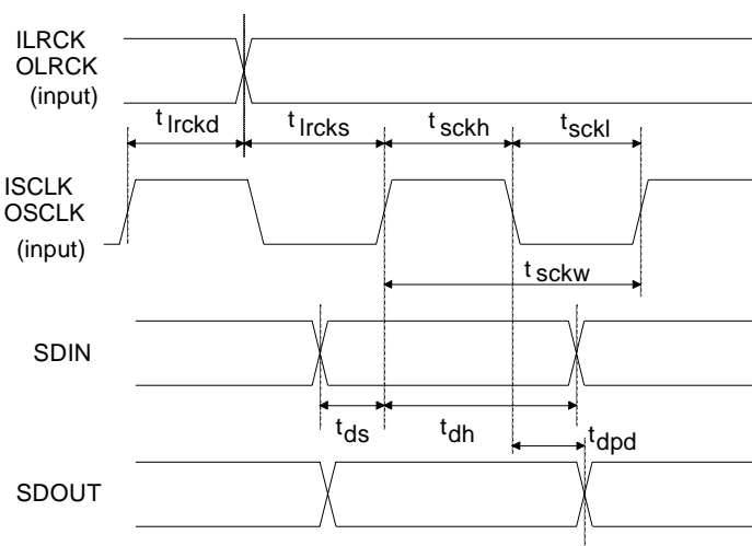
Figure 2. Audio Ports Slave Mode and Data I/O Timing
