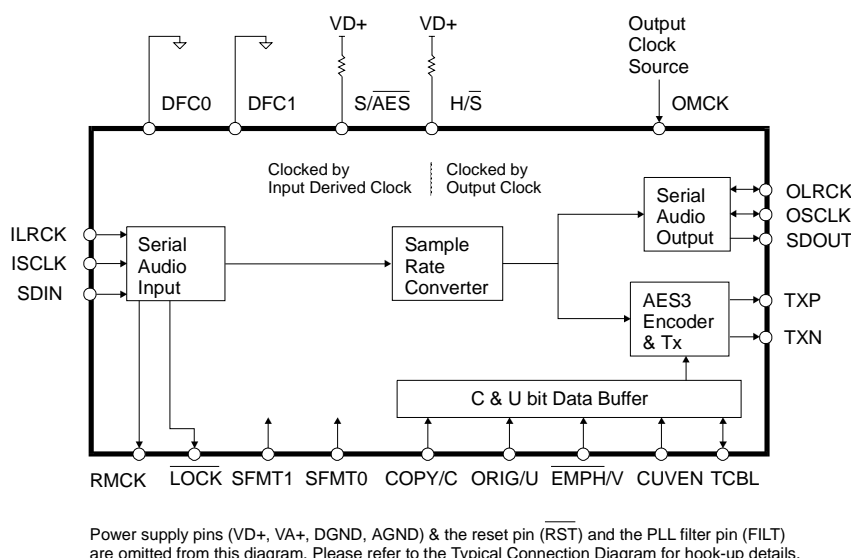
Figure 27. Hardware Mode 2 - Default Data Flow, Serial Audio Input
