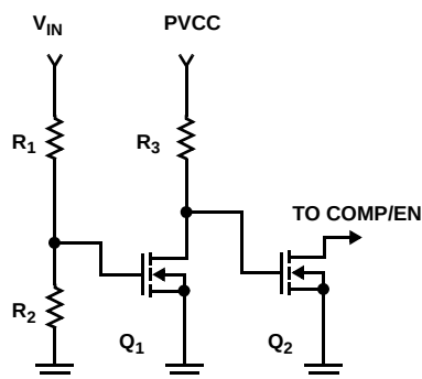
FIGURE 20. SEQUENCE CIRCUIT
