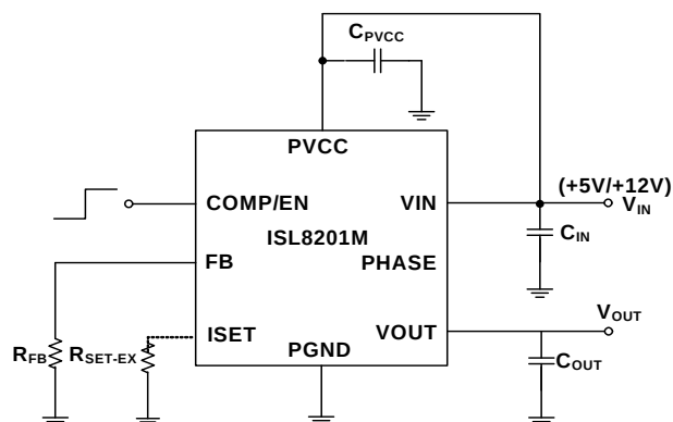
FIGURE 11. TYPICAL APPLICATION SCHEMATIC
