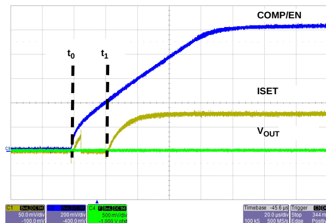
FIGURE 14. I_{SET} AND SOFT-START OPERATION
