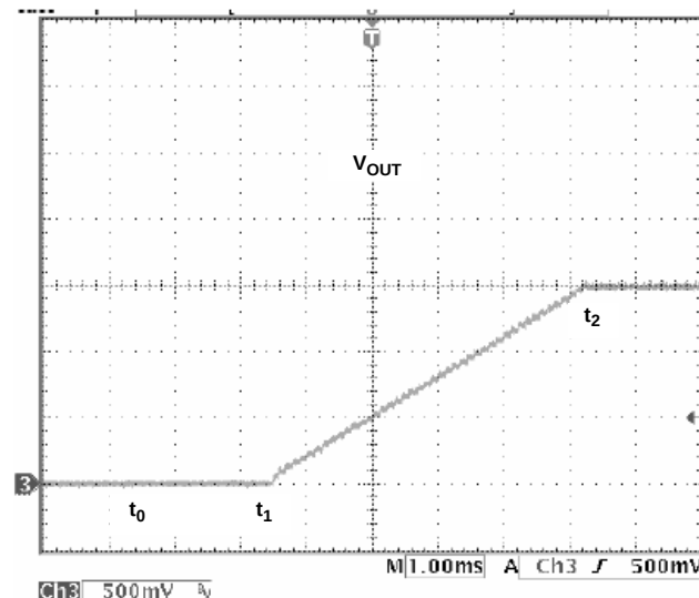
FIGURE 16. NORMAL START-UP
