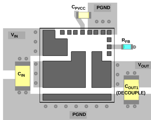
FIGURE 21. RECOMMENDED LAYOUT
