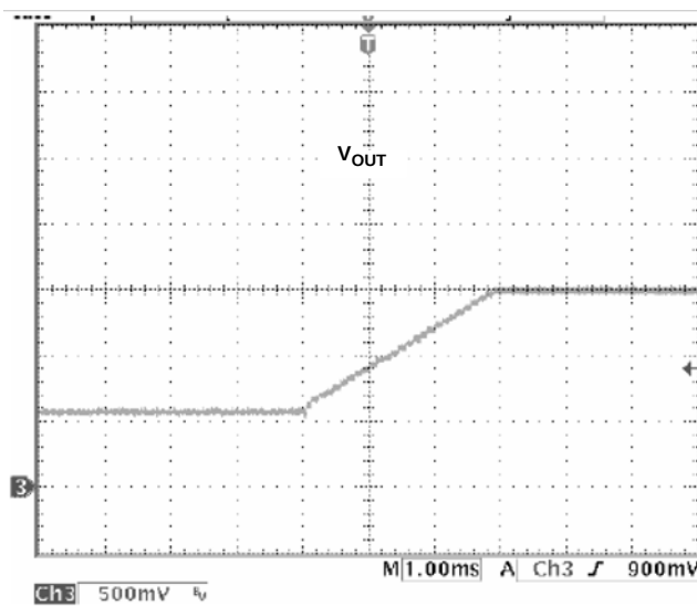
FIGURE 17. PRE-BIASED START-UP
