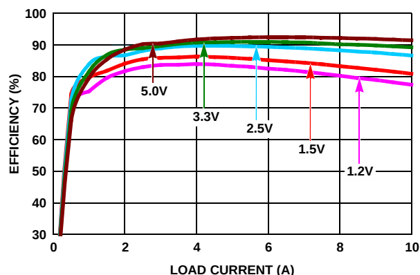
FIGURE 4. EFFICIENCY vs LOAD CURRENT ( 18V_{IN} )
