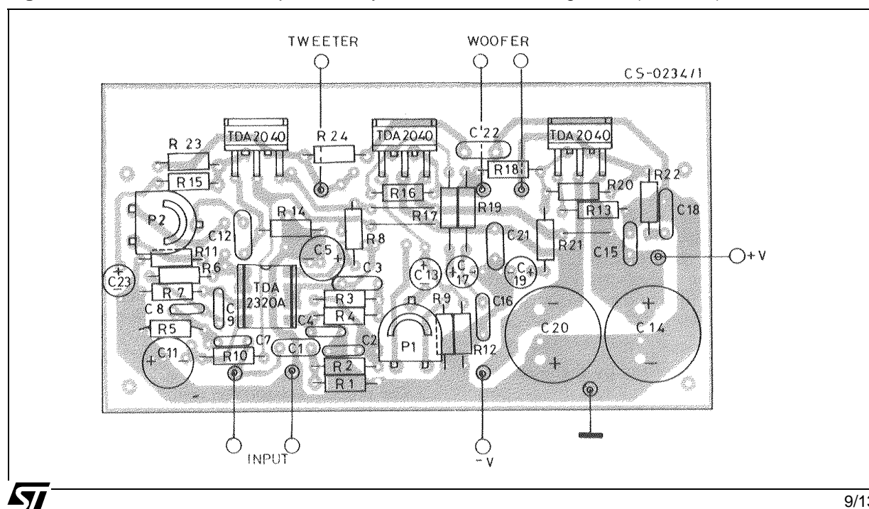
Figure 17 : P.C. Board and Components Layout for the Circuit of Figure 16 (1:1 scale)
