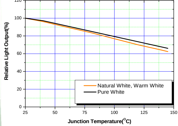
Relative Light Output vs. Junction Temperature at IF=20mA
