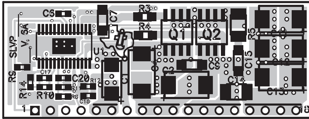
Top Assembly
