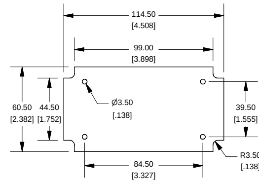
SIDE VIEW OF ENCLOSURE
