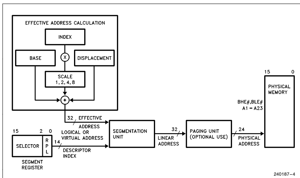
Figure 2.3. Address Translation
