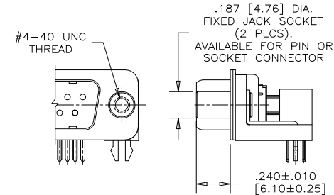
PARTIAL FRONT VIEW
