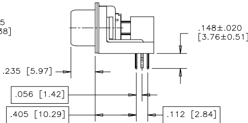
PARTIAL FRONT VIEW
