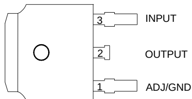
(TO-252-2 (3) (Option 2))
