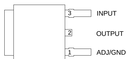
(TO-252-2 (5))
