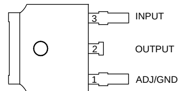
D Package (TO-252-2 (3) (Option 1))
