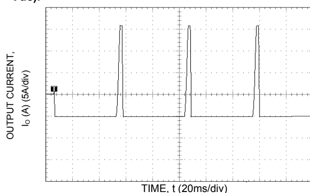
Figure 18. Output short circuit Current ( V_{in} = 12\text{Vdc} , V_o = 0.75\text{Vdc} ).
