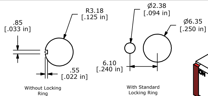
PANEL MOUNTING
