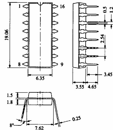
16-Lead DIL Plastic Package (16-DIP)
