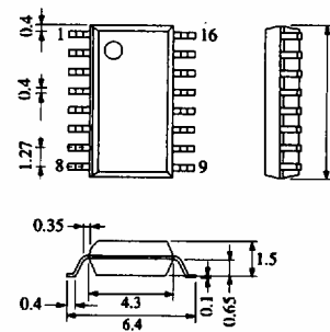
16-Lead PANAFLAT Plastic Package (SO-16D)
