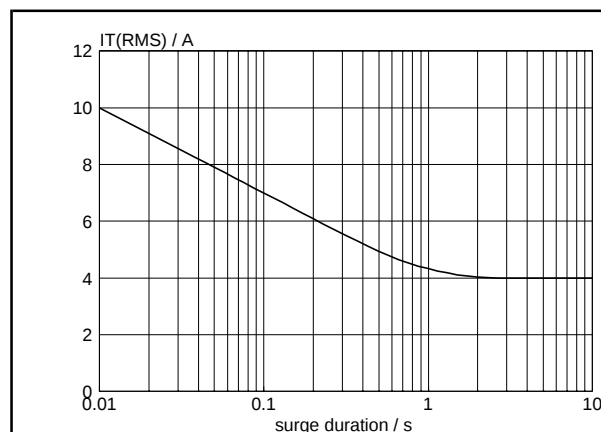
Fig.5. Maximum permissible repetitive rms on-state current I_{T(RMS)} , versus surge duration, for sinusoidal currents, f = 50\text{ Hz} ; T_{mb} \leq 107^\circ\text{C} .
