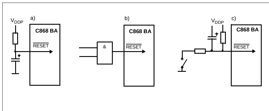
Figure 10 Reset Circuitries
